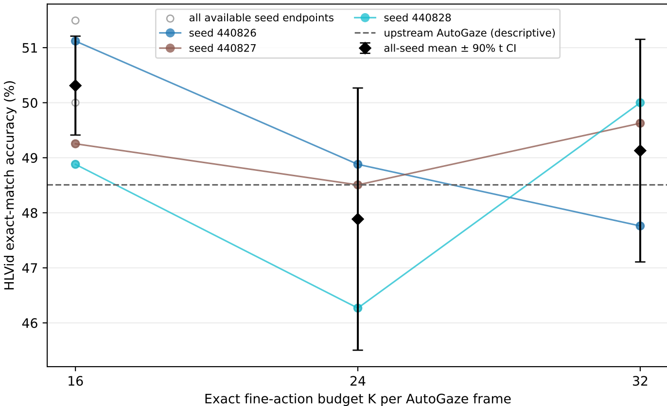
Human-gaze AutoGaze transfer under NVILA MTV48
