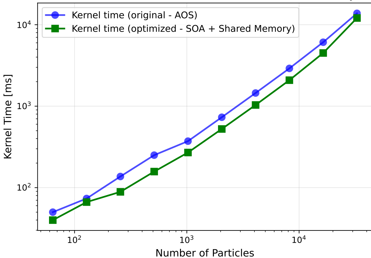
Kernel Performance: AOS vs SOA + Shared Memory
