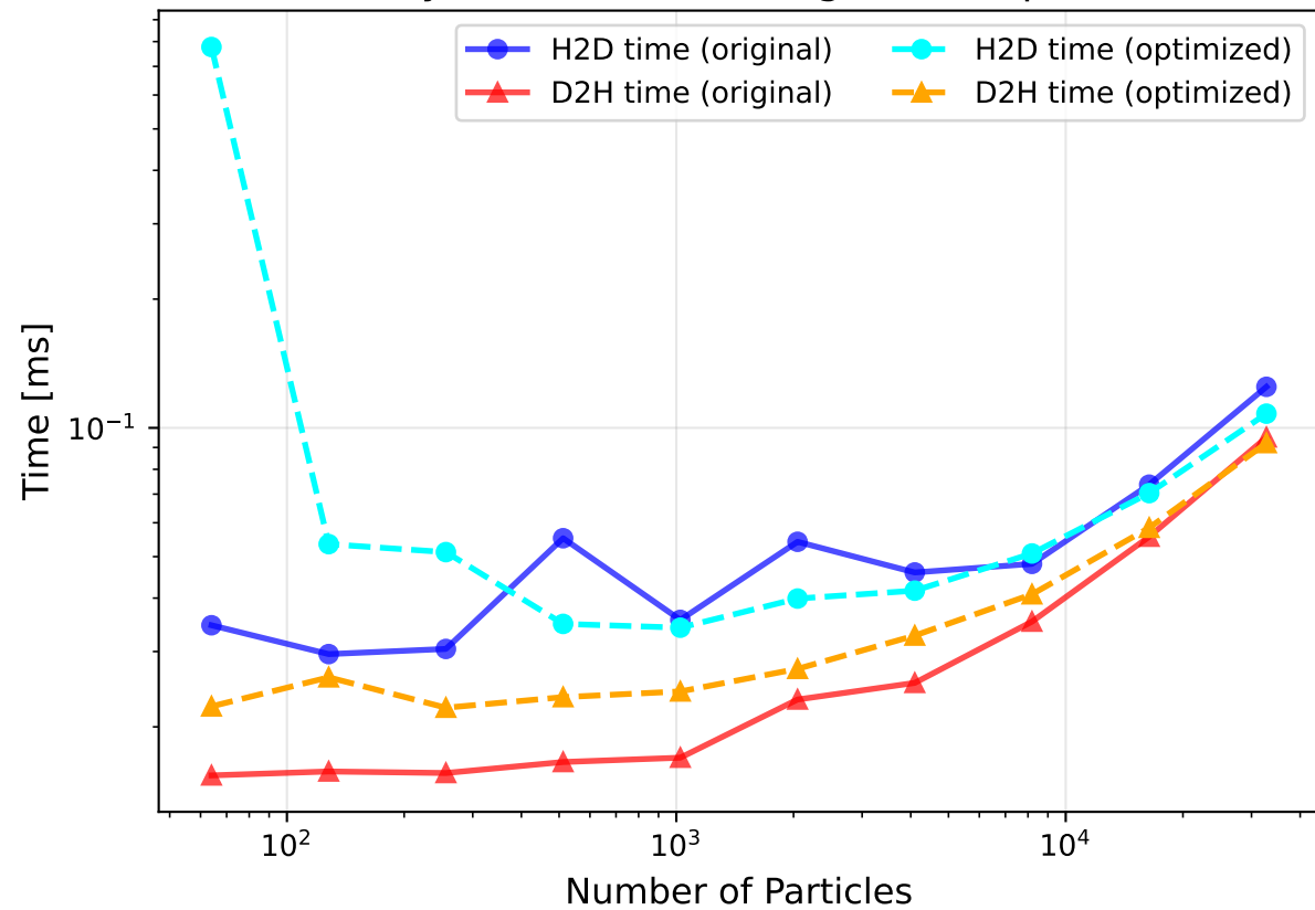
Memory transfer time: Original vs Optimized
