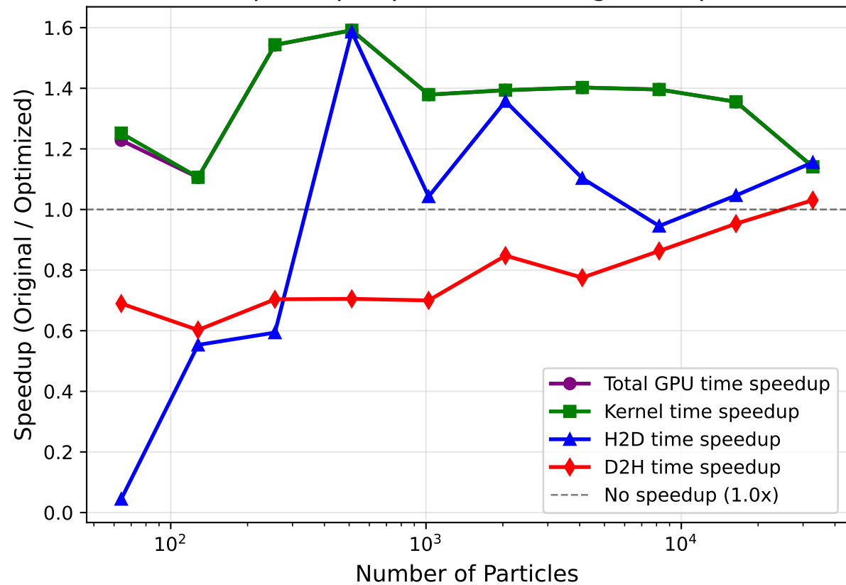
Performance Speedup: Optimized vs Original Implementation
