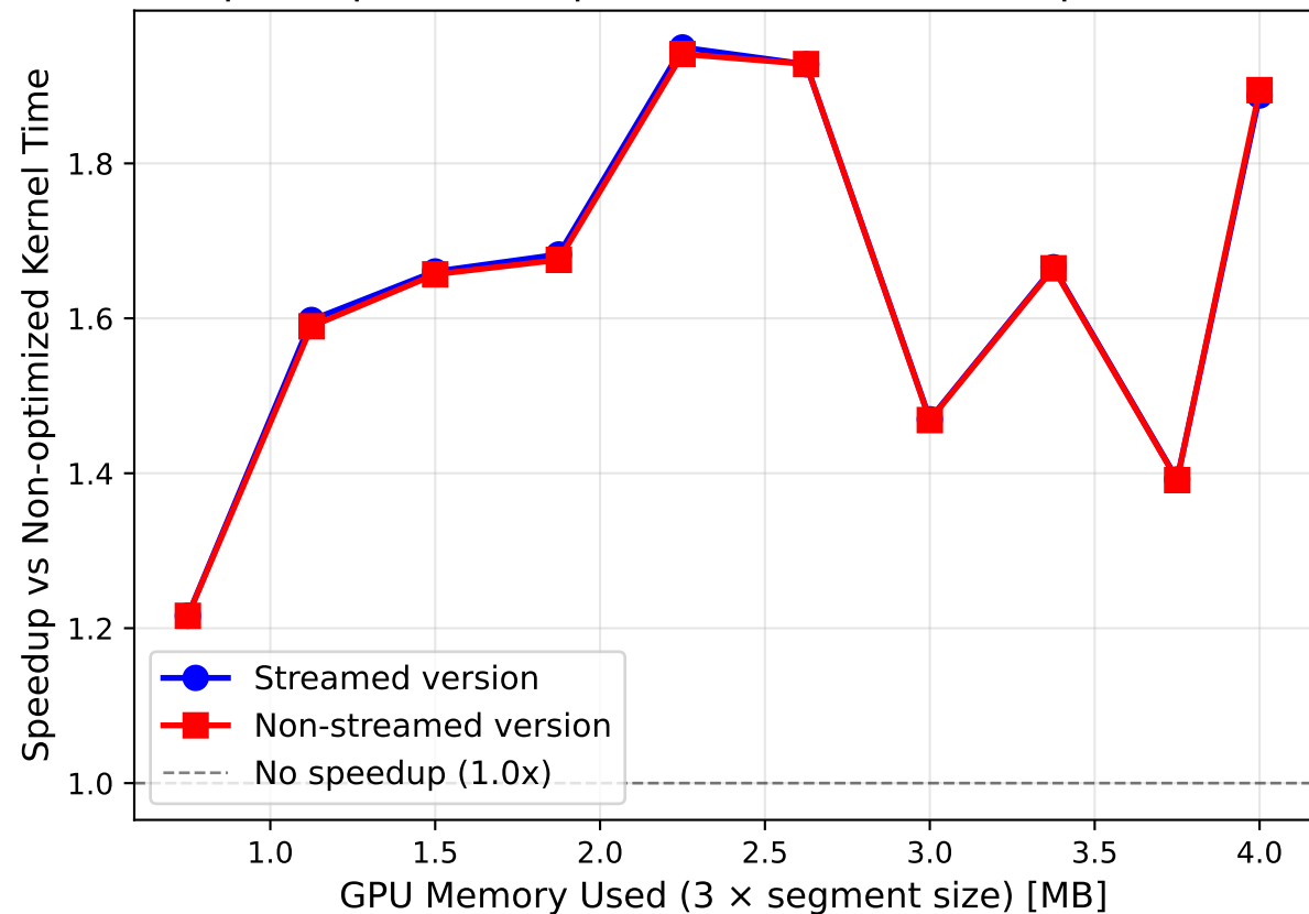
Speedup vs Non-optimized Version (512k particles)
