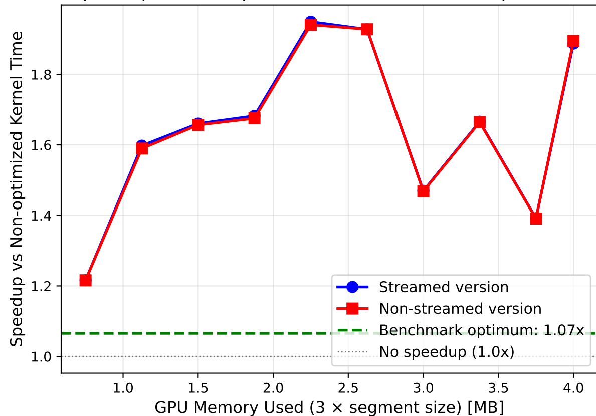
Speedup vs Non-optimized Benchmark (512k particles)
