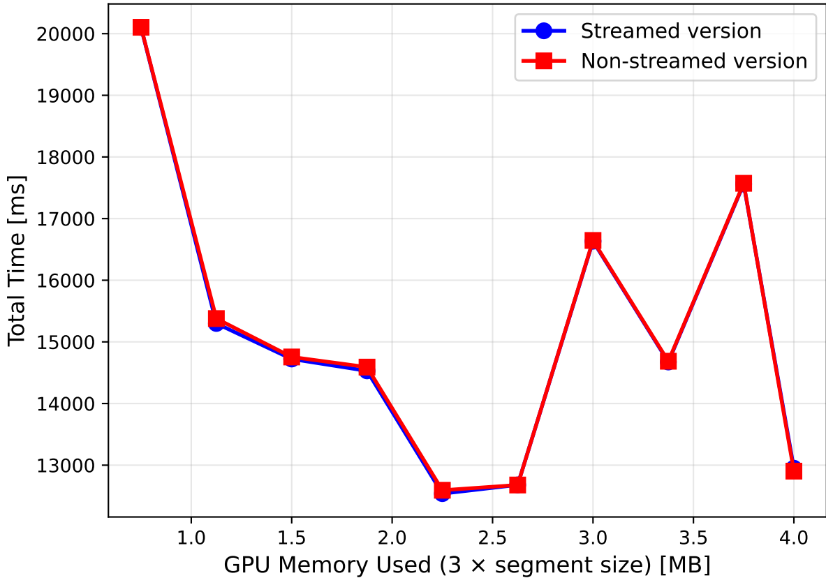
Streamed vs Non-streamed: Performance vs GPU Memory Usage (512k particles)
