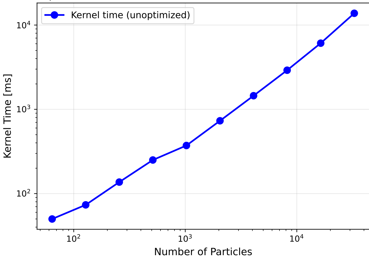
Unoptimized Benchmark: Kernel Time vs Number of Particles
