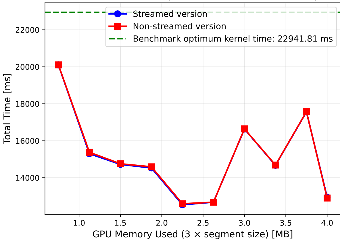
Total Time vs Benchmark Optimum Kernel Time (512k particles)
