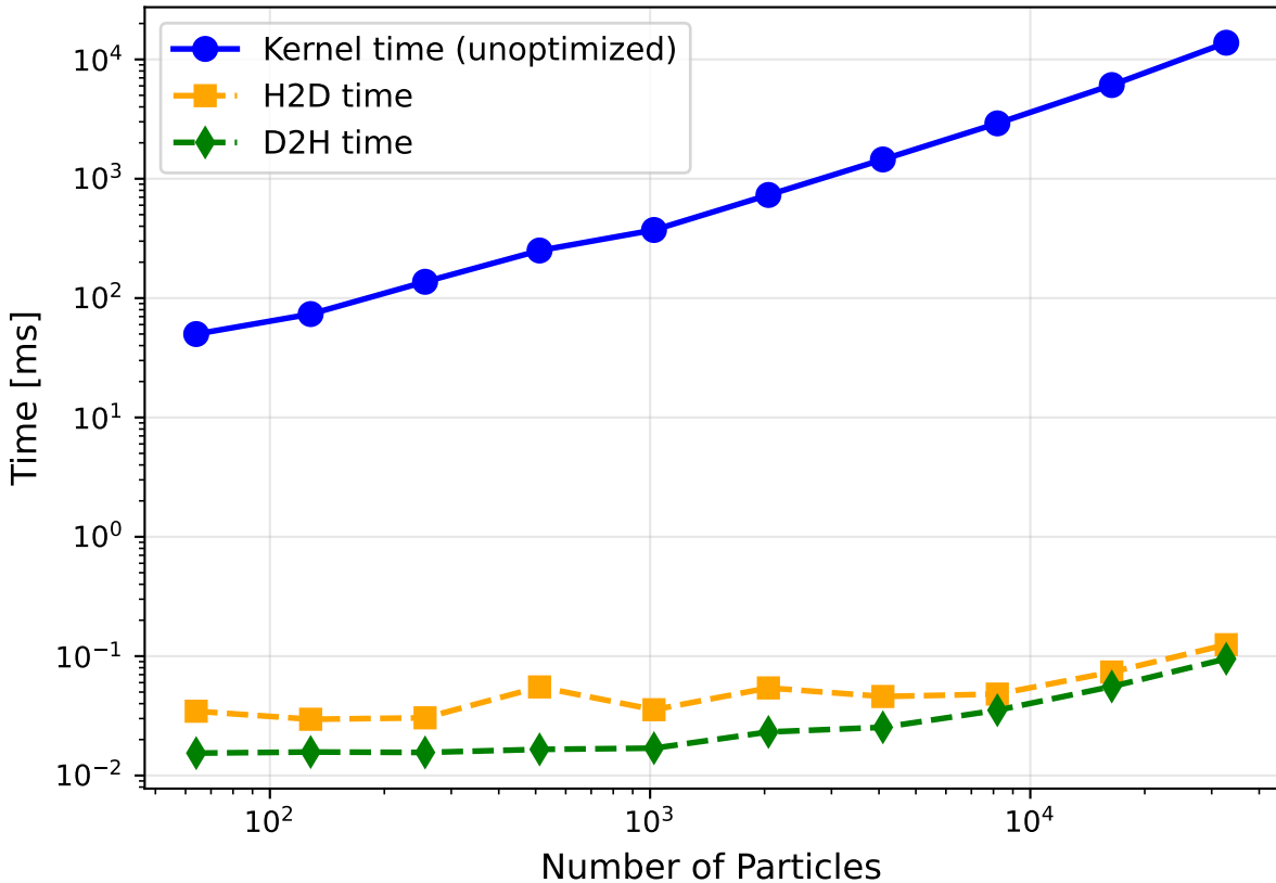
Unoptimized Benchmark: Kernel, H2D, and D2H Times vs Number of Particles
