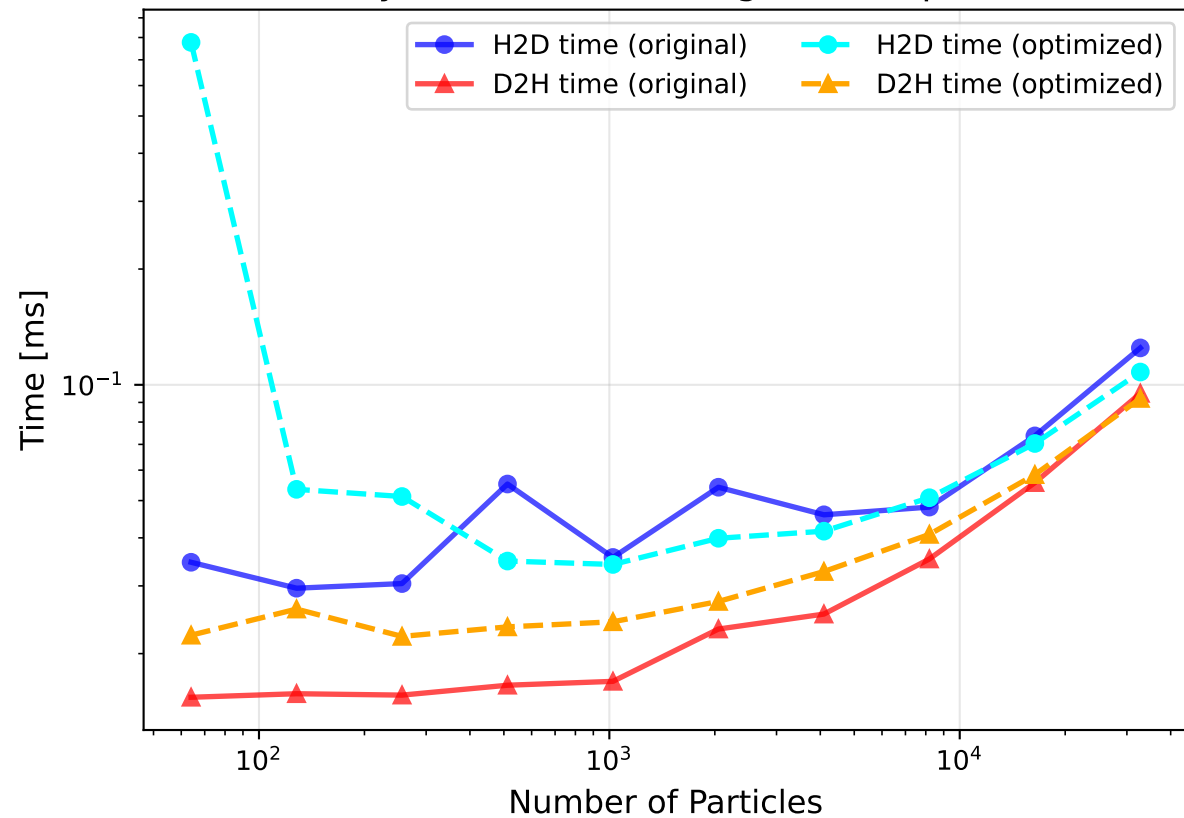
Memory transfer time: Original vs Optimized
