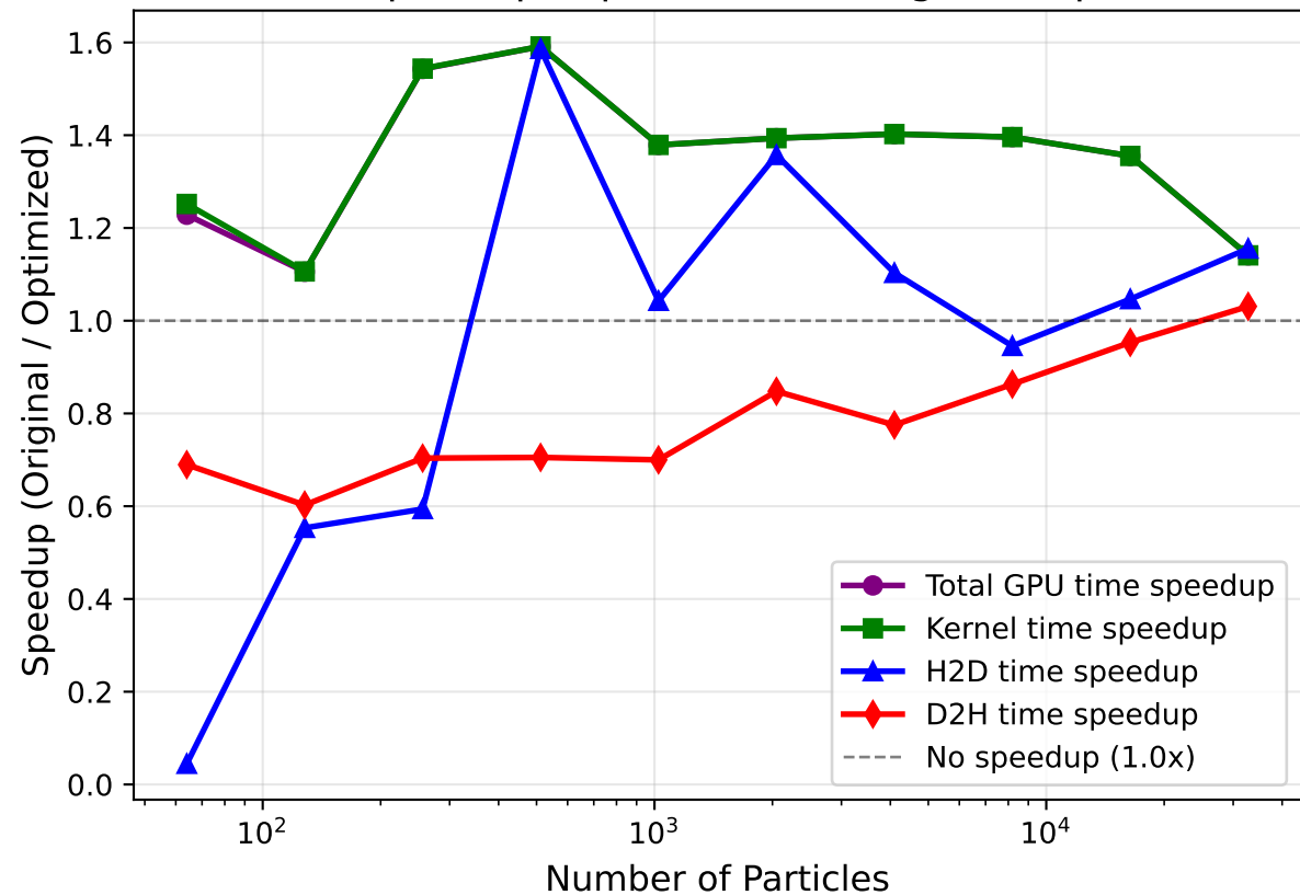
Performance Speedup: Optimized vs Original Implementation
