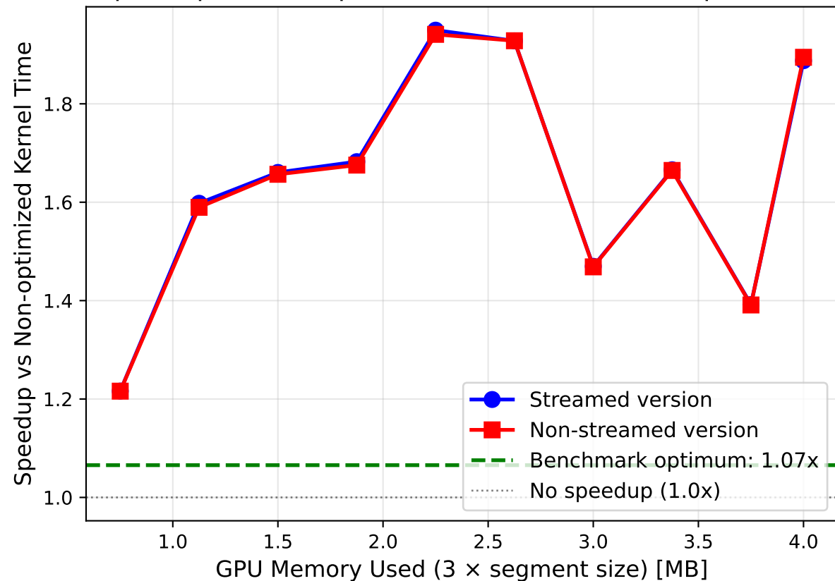
Speedup vs Non-optimized Benchmark (512k particles)
