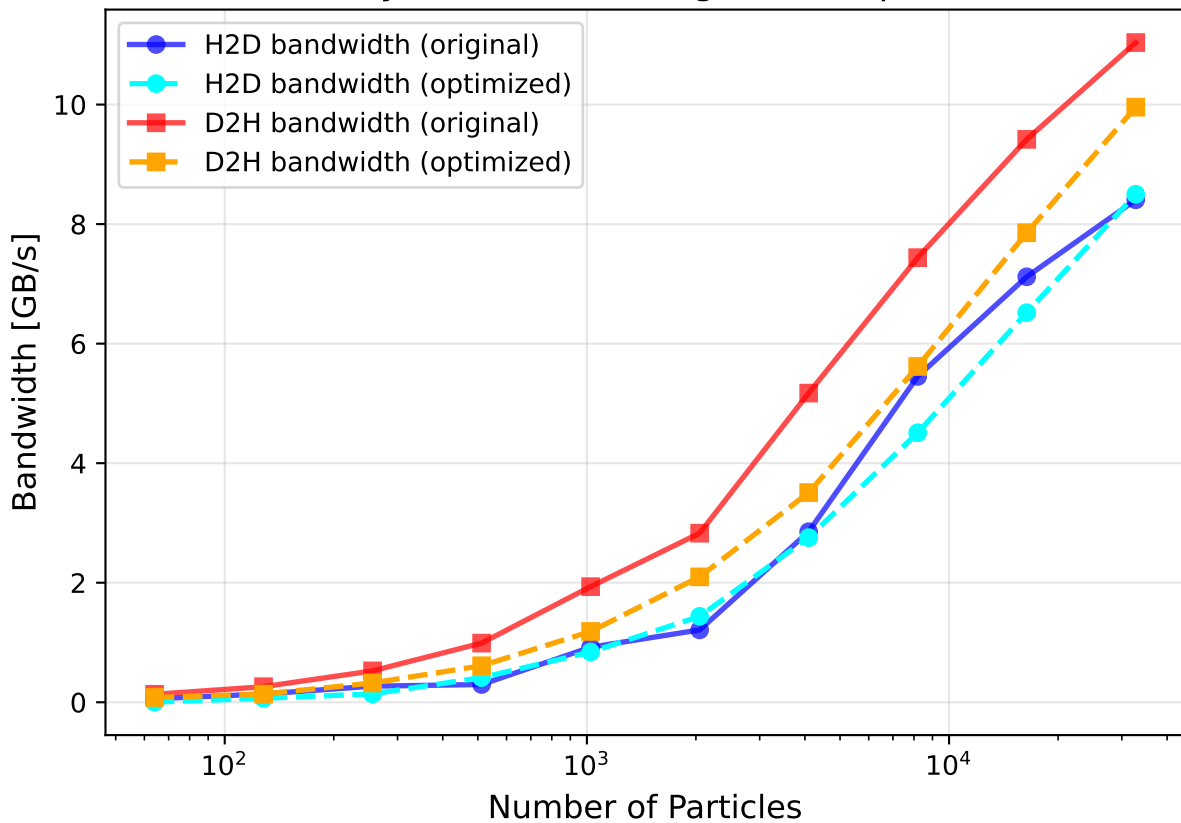
Memory Bandwidth: Original vs Optimized
