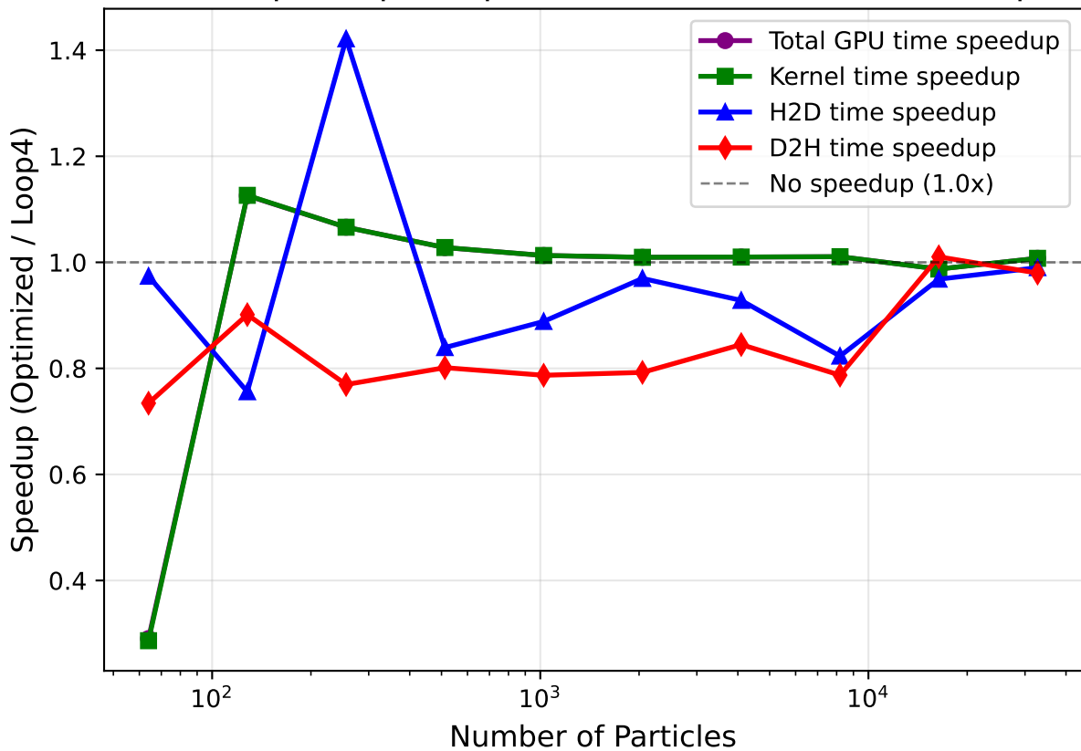
Performance Speedup: Loop Unroll Factor 4 vs Standard Optimized
