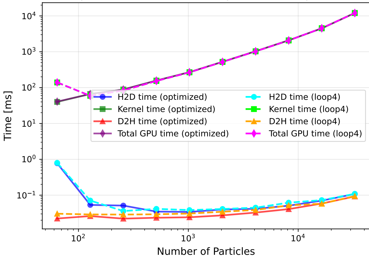
GPU Time: Optimized (Standard) vs Optimized (Loop Unroll Factor 4)
