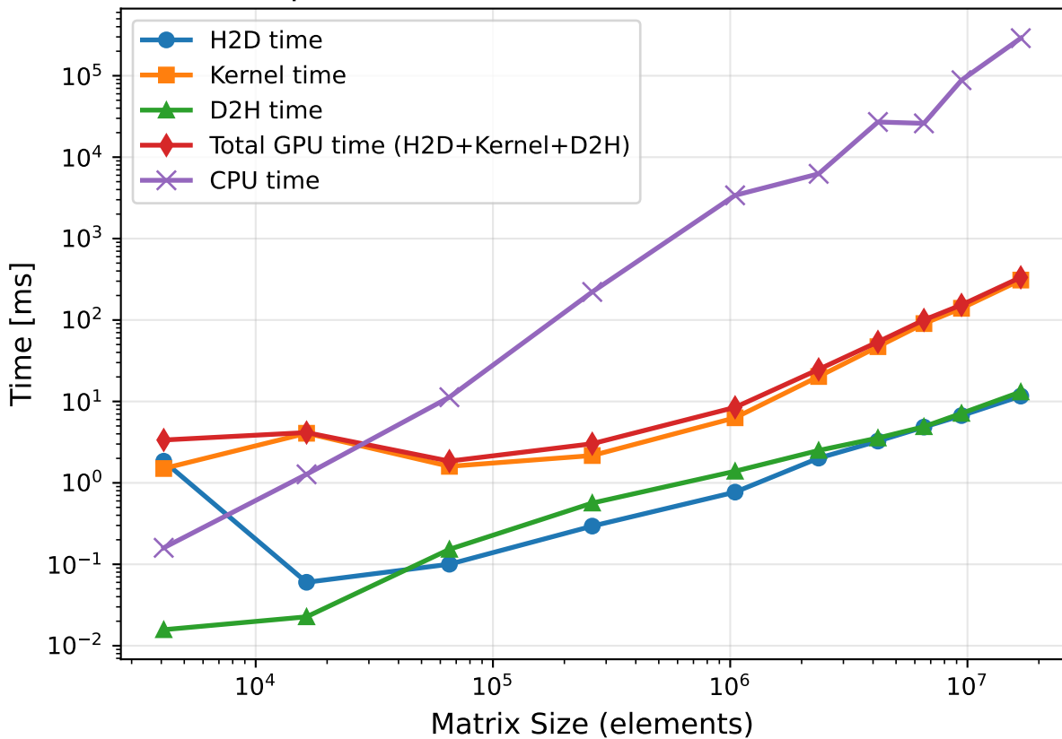
Matrix Multiplication Performance: GPU vs CPU (32 threads)
