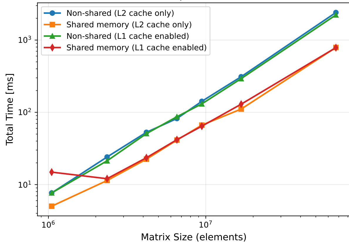
Performance comparison L1 vs L2 cache
