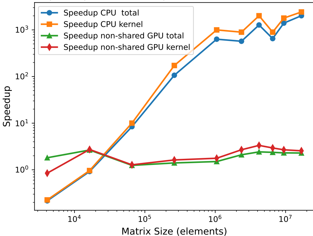
Speedup of shared implementation (32 threads)
