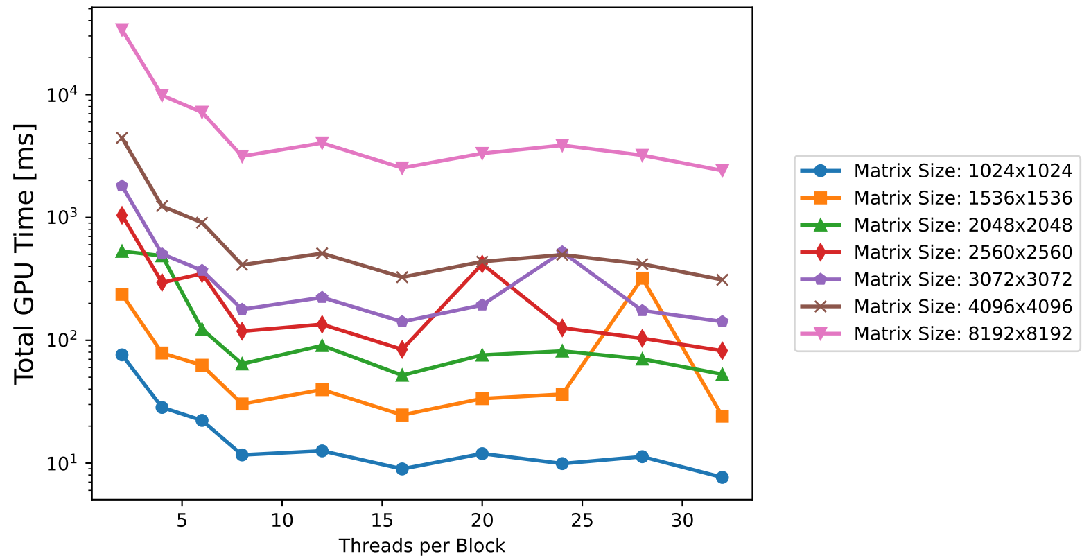
Total GPU Time (H2D + Kernel + D2H)
