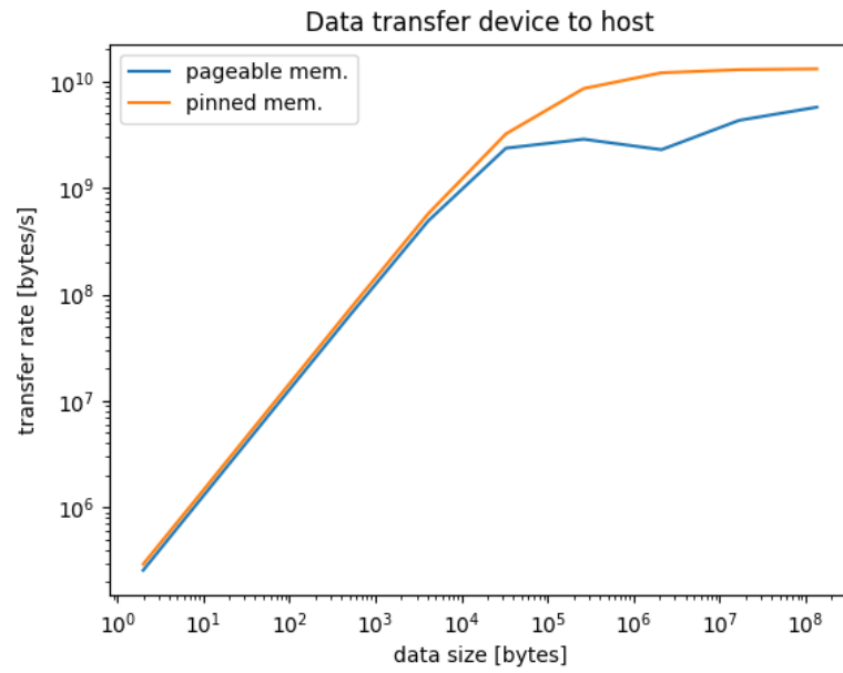
Figure 4: Device to Host: pinned vs. pageable memory
