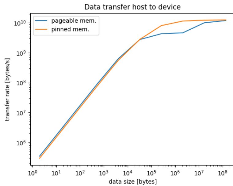
Figure 5: Host to Device: pinned vs. pageable memory
