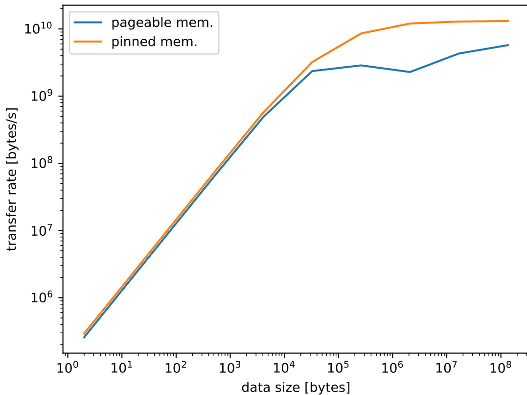
Data transfer device to host
