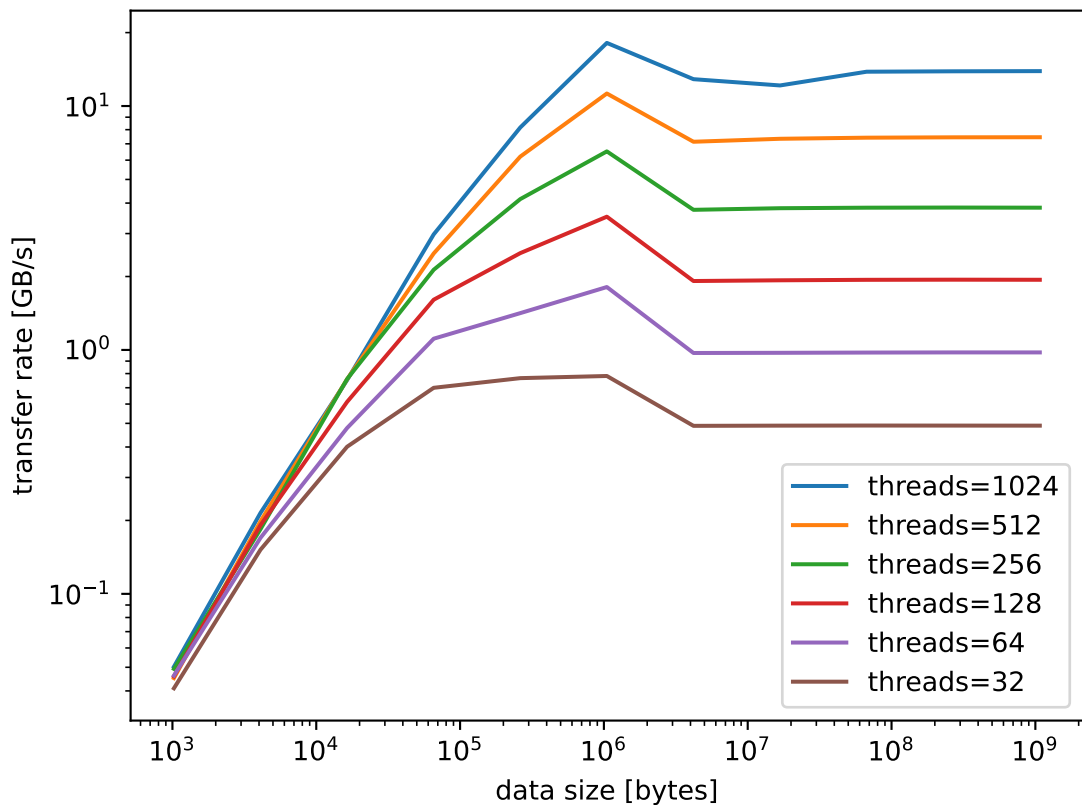
coalesced thread access with one threadblock
