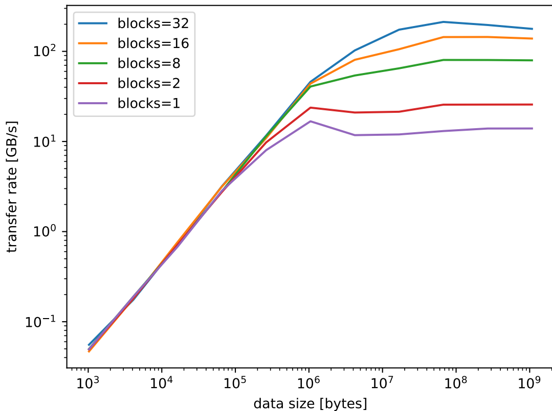
coalesced thread access with 1024 threads
