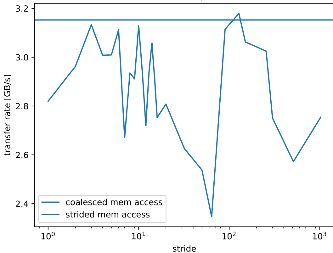
strided memory access
