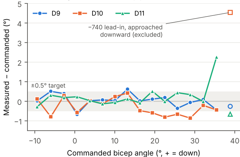
(a) Joint angle error, on-axis Up pass
