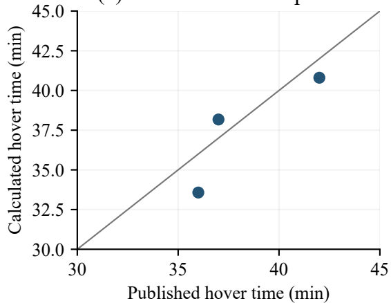
(b) Three-aircraft comparison
