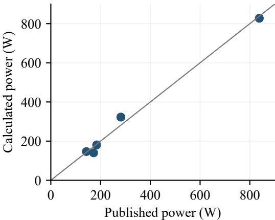
(a) Five-point hover fit
