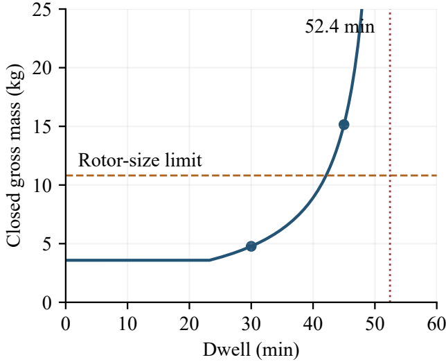
Figure 5. Reference carrier mass versus dwell, evaluated from the stated branch equations. The rotor screen binds at 42.1 minutes; the energy slope reaches one at 52.4 minutes. The plotted finite curve is clipped at 25 kg for readability.
