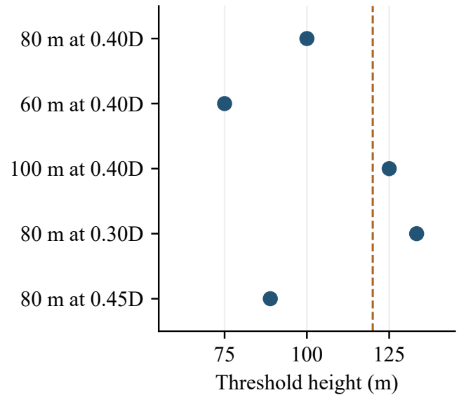
Figure 6. Relay height at which the first hop begins to clear, for the five screen cases. Thresholds above 120 m remove that altitude layer from service, while changes that stay between 60 and 120 m leave the sampled results unchanged. This comparison is geometric; no terrain model underlies it.
