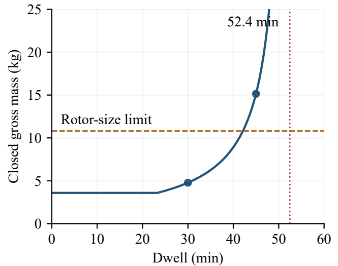
Figure 5. Reference carrier mass versus dwell, evaluated from the stated branch equations. The rotor screen binds at 42.1 minutes; the energy slope reaches one at 52.4 minutes. The plotted finite curve is clipped at 25 kg for readability.
