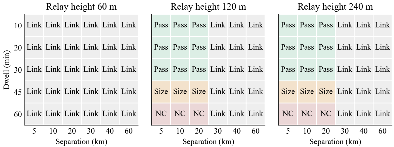
Figure 4. Baseline results for the 90 primary cases. PASS means the relay helps and the aircraft stays within the screening limits, SIZE marks a solution outside those limits, NC marks a case with no solution, and LINK FAIL marks the earlier link check. All cells in the 60 m panel fail visibility. Link failures in the 120 m and 240 m panels are clear but short of margin. No case in the baseline is direct-sufficient.
