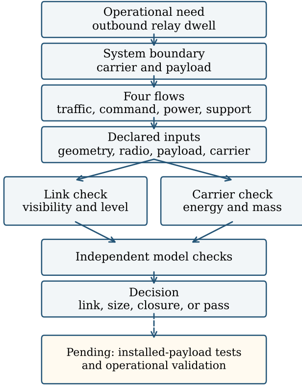
Figure 2. Architecture assessment workflow. The service need and four allocated flows lead to declared inputs, parallel link and carrier checks, and independent model review. Failure labels identify which architecture assumption or resource needs reconsideration. Installed-payload tests and operational validation remain outstanding.
