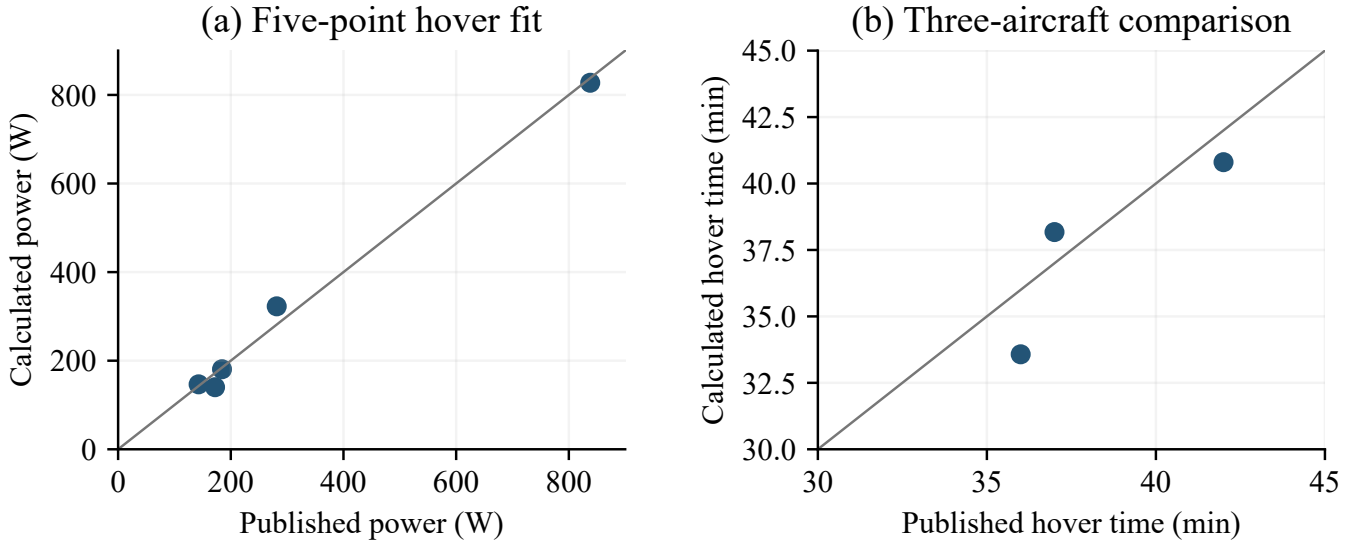
Figure 3. Hover evidence shown on separate axes. Left: measured and fitted electrical powers for the five NASA points. Right: published and calculated maximum-hover times for three aircraft excluded from the fit. A diagonal indicates agreement; neither panel validates carrier mass closure.
