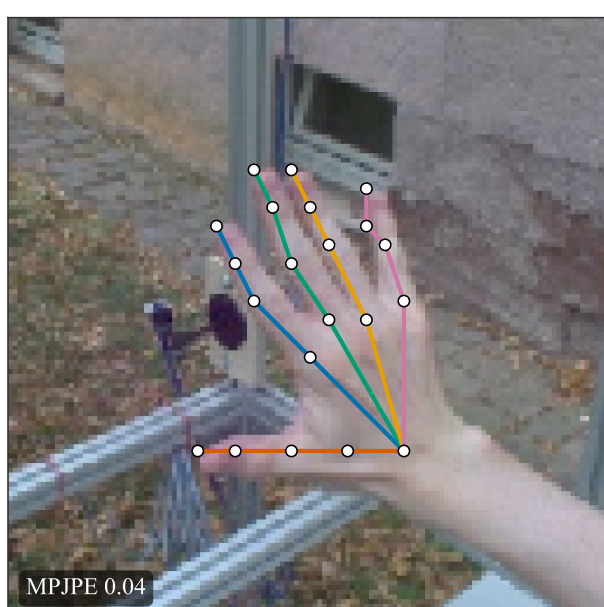
L1 – 55% AUC 66.76%
