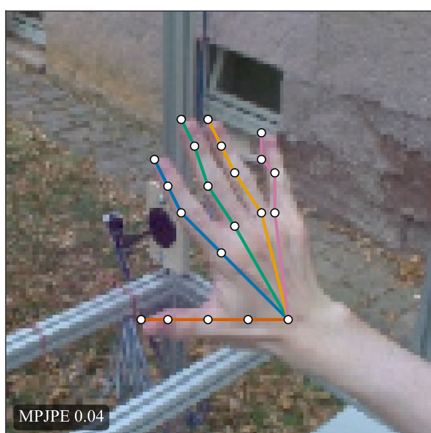
Taylor – 55% AUC 66.52%
