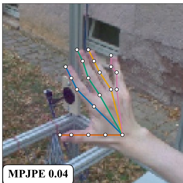
Taylor – 55% AUC 66.52%
