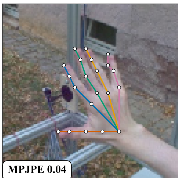
L1 – 55% AUC 66.76%
