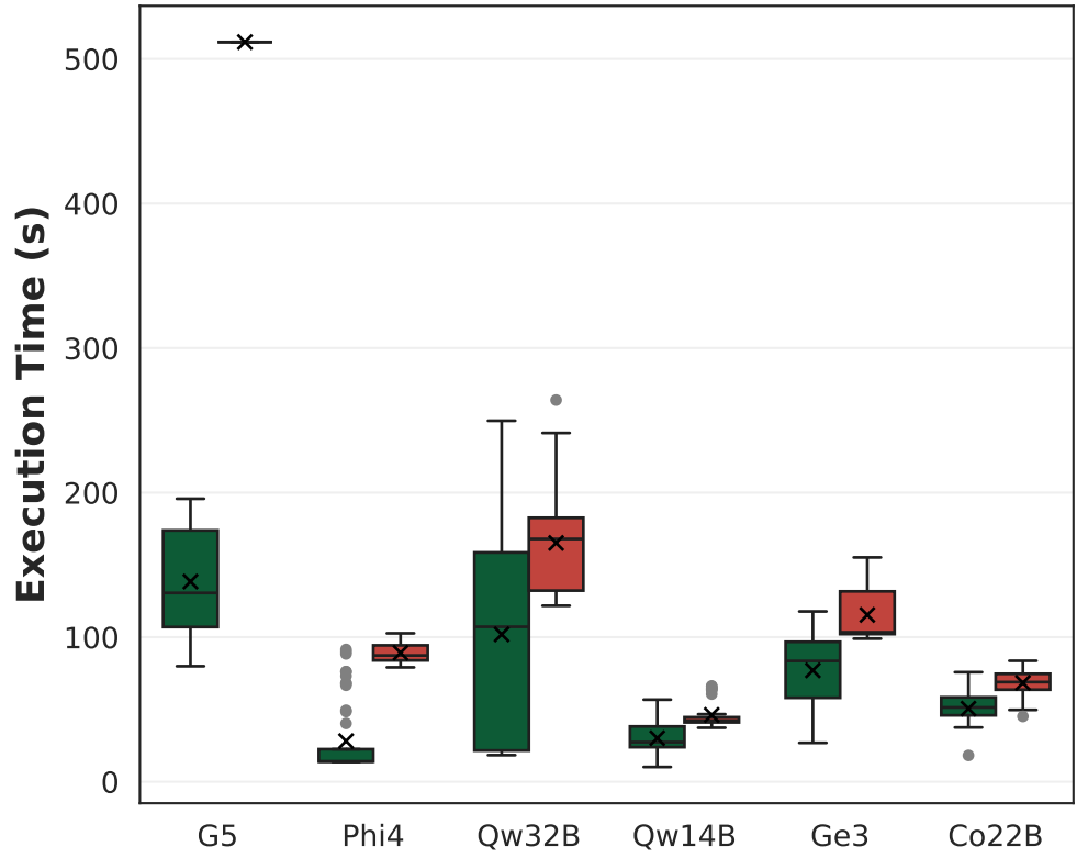
Python Sketch Generation on CPU
