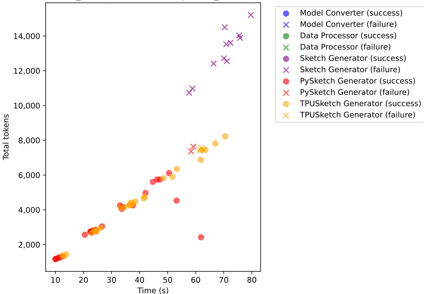
Time vs Tokens phi4:14b_5f04, params{None} | 02.06_abla-l2-phi4
