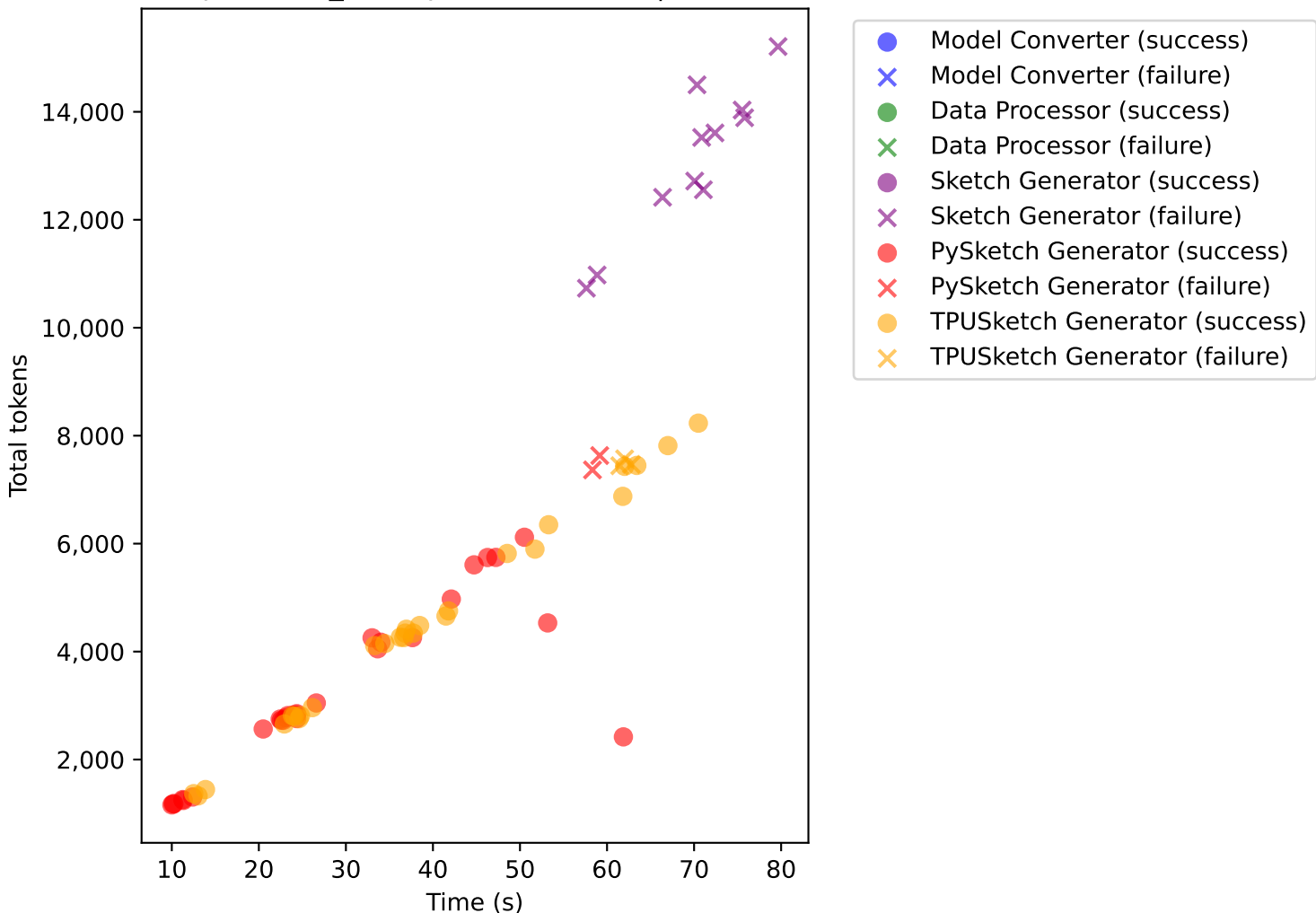
Time vs Tokens phi4:14b_5f04, params{None} | 02.06
