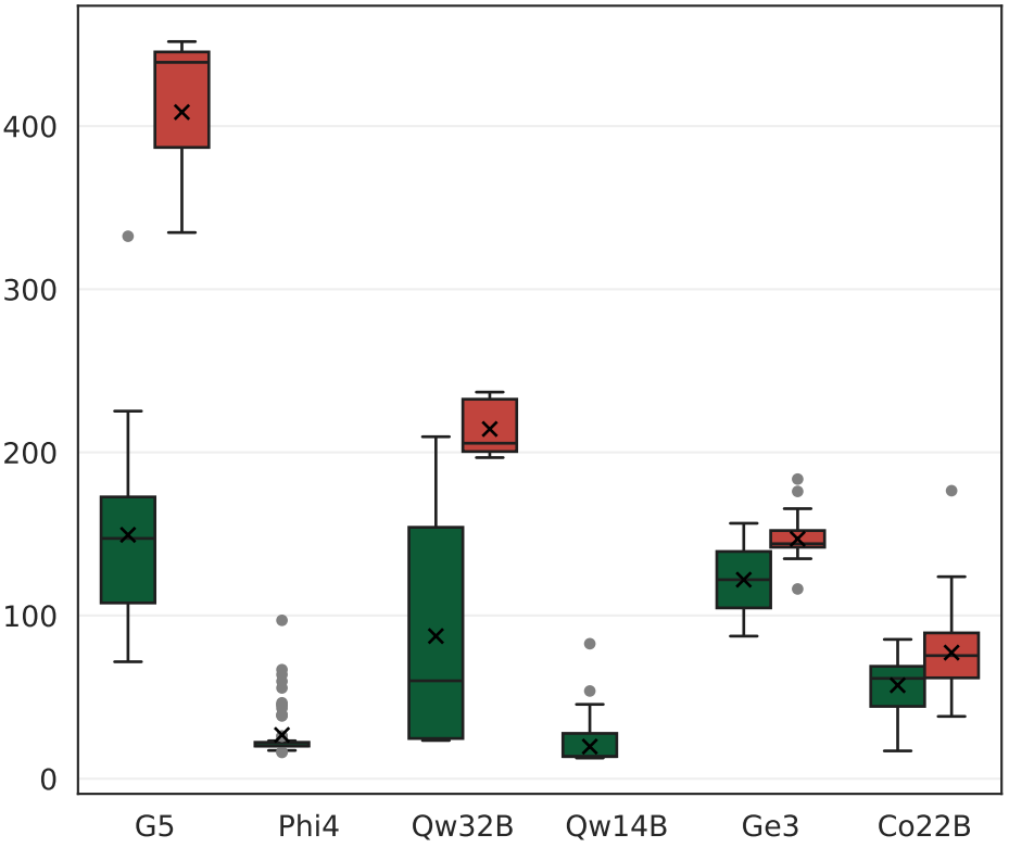
Python Sketch Generation on TPU
