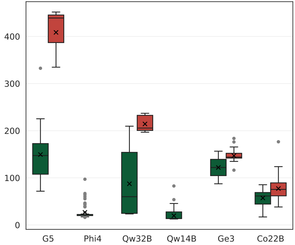
Python Sketch Generation on TPU
