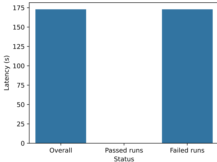
Sketch Generator
