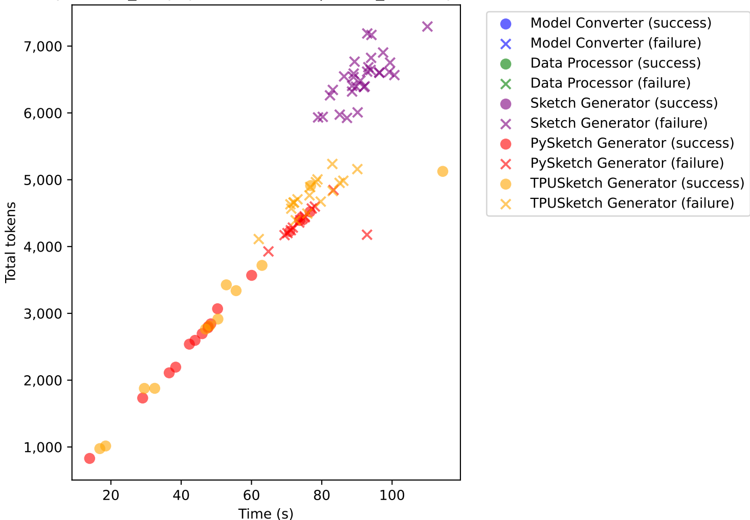
Time vs Tokens phi4:14b_ab1p, params{None} | 02.05_abla-l1-phi4
