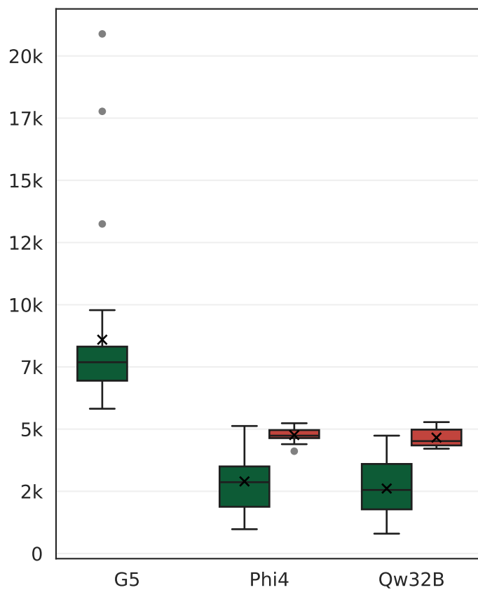
# Tokens (Total)
