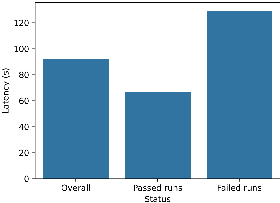
TPUSketch Generator
