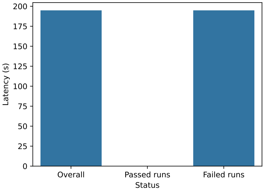
Sketch Generator
