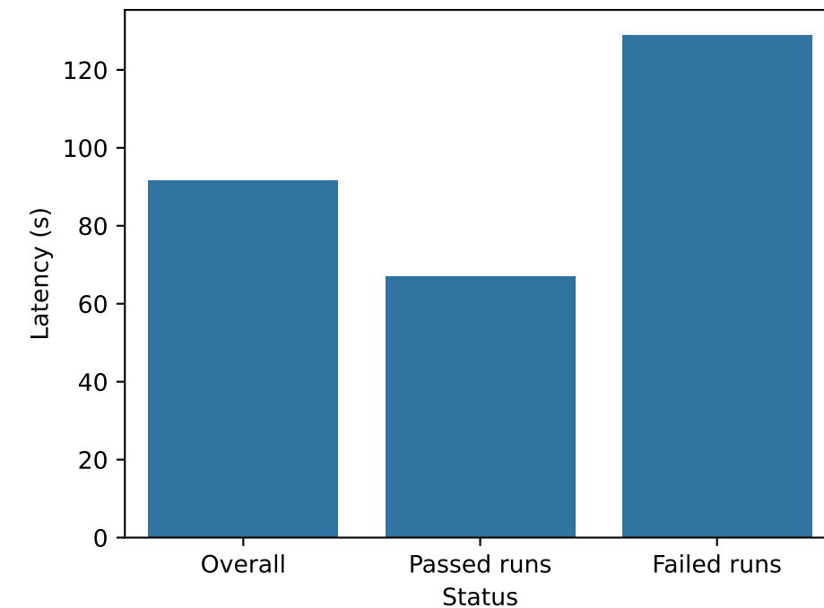
TPUSketch Generator
