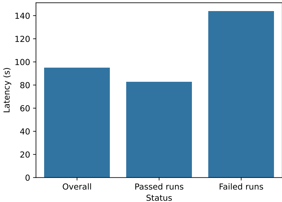
TPUSketch Generator
