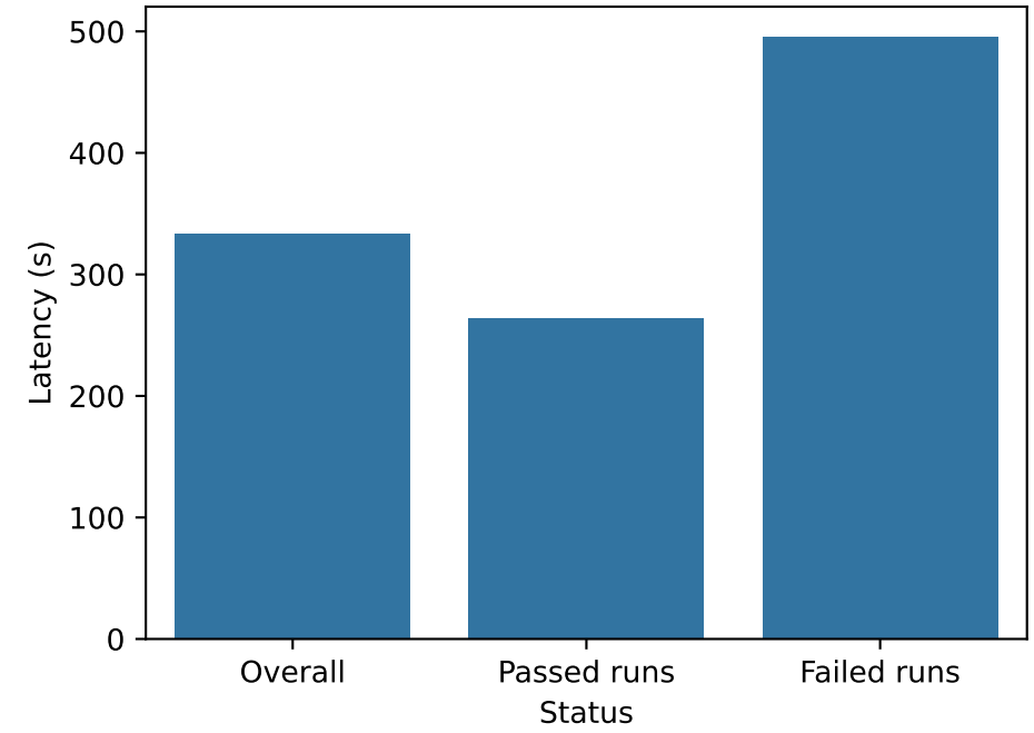
Sketch Generator
