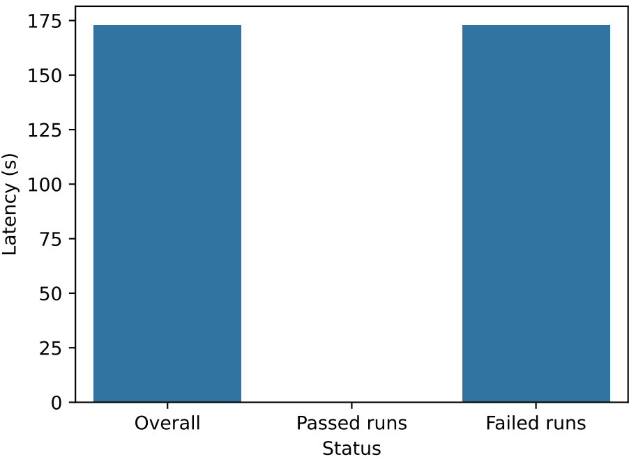
Sketch Generator
