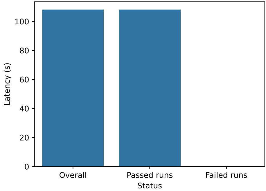
TPUSketch Generator
