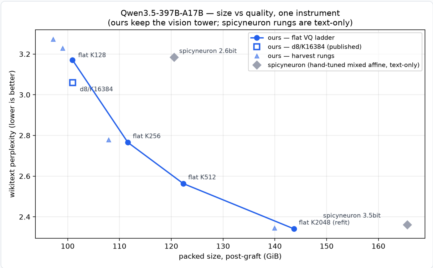
397B ladder
