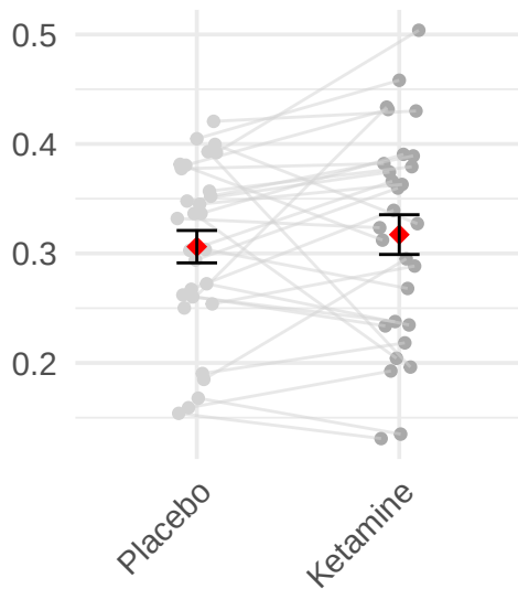
Saliency
