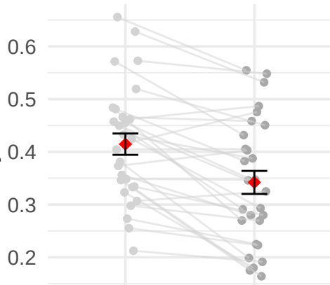
Saliency
