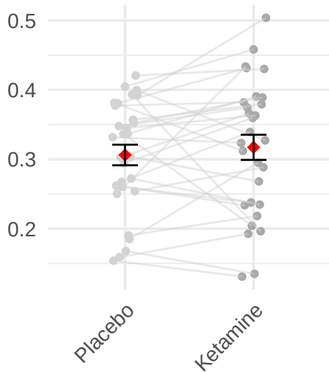
Saliency
