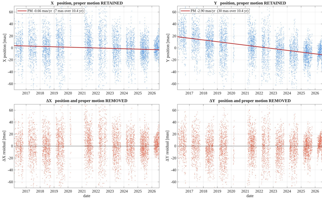
Figure 4. BLG01 — unbinned, one point per exposure, no error bars. Columns are the two axes, X left and Y right . Top row: the measured position with the proper motion retained ; the red line is the fitted proper motion. Bottom row: the same with position and proper motion removed. All four panels share one vertical scale so the axes can be compared directly; it is set from the robust scatter, so a handful of extreme points fall outside it. Positions are relative to the target's own mean.
