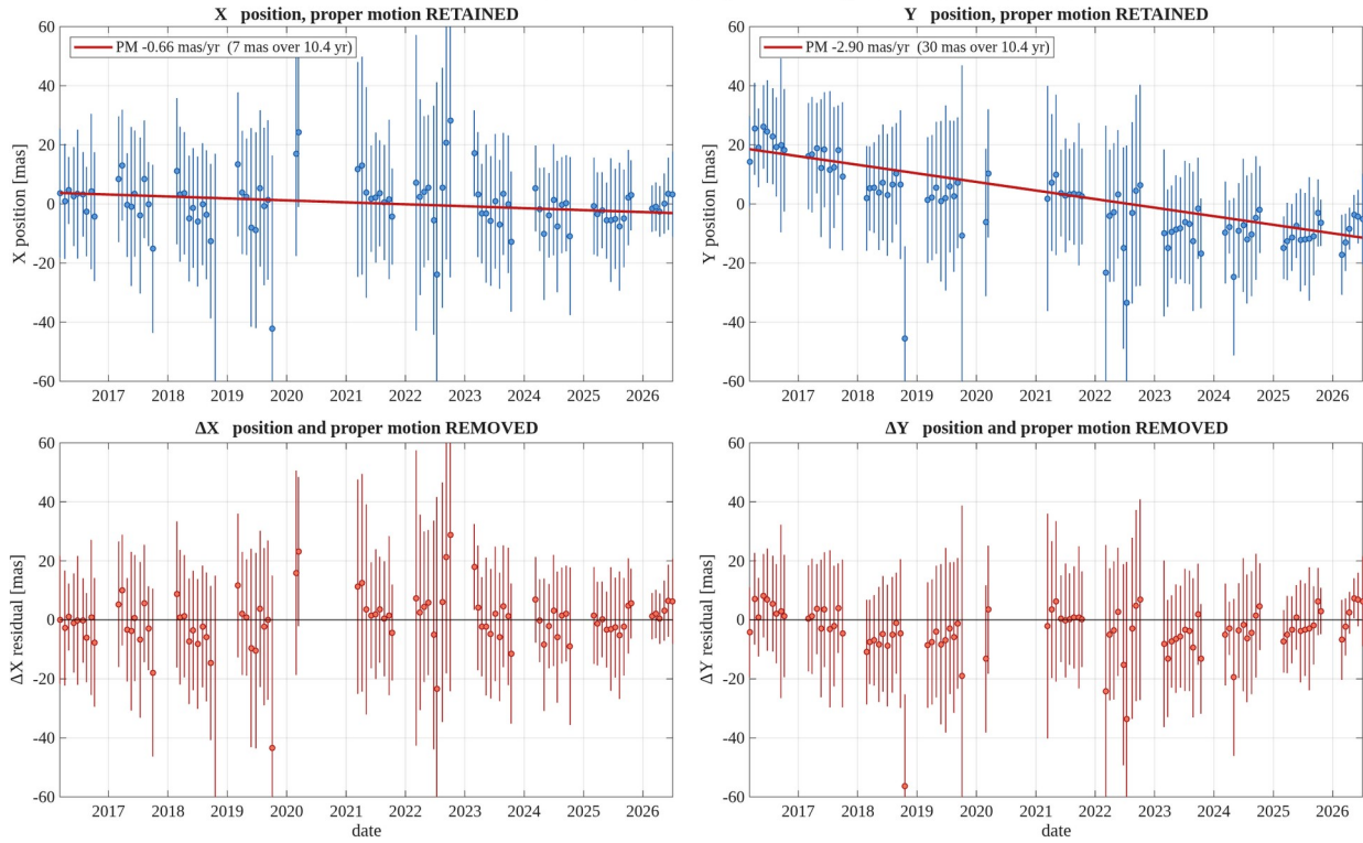
Figure 5. BLG01 — binned in one sidereal month (27.321661 d); error bars are the RMS within the bin. Columns are the two axes, X left and Y right . Top row: the measured position with the proper motion retained ; the red line is the fitted proper motion. Bottom row: the same with position and proper motion removed. All four panels share one vertical scale so the axes can be compared directly; it is set from the robust scatter, so a handful of extreme points fall outside it. Positions are relative to the target's own mean.
