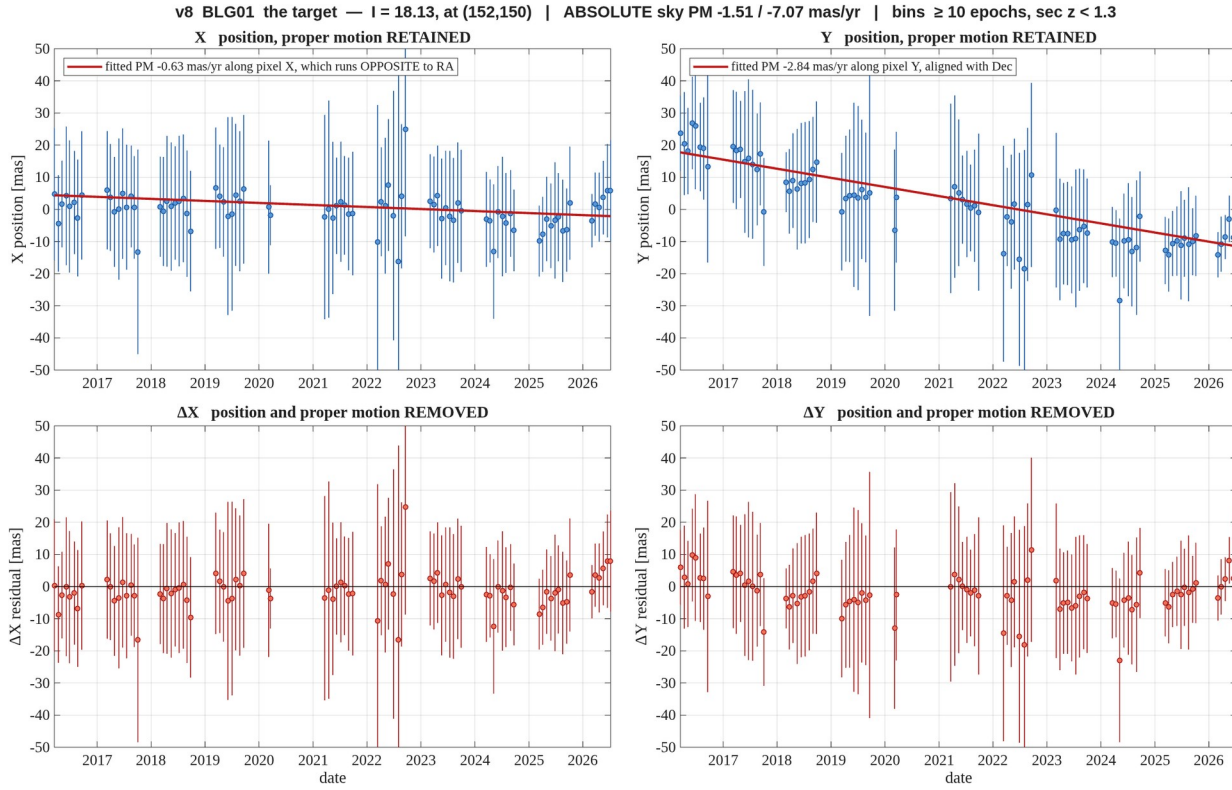
Figure 16. BLG01 — the target, l = 18.13 . Binned in one sidereal month, error bars are the RMS within the bin; bins with fewer than 10 epochs and epochs at sec z > 1.3 are dropped. Columns are the two axes, X left and Y right ; the top row keeps the proper motion, the bottom row removes it. The heading gives the absolute sky motion with the full gauge removed; the legend gives it along the pixel axis, and pixel X runs opposite to RA , so the two carry opposite signs in X.
