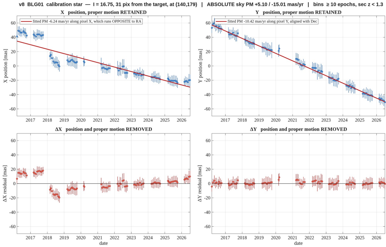
Figure 22. BLG01 — l = 16.75 , 31 pix away. Binned in one sidereal month, error bars are the RMS within the bin; bins with fewer than 10 epochs and epochs at sec z > 1.3 are dropped. Columns are the two axes, X left and Y right ; the top row keeps the proper motion, the bottom row removes it. The heading gives the absolute sky motion with the full gauge removed; the legend gives it along the pixel axis, and pixel X runs opposite to RA , so the two carry opposite signs in X.
