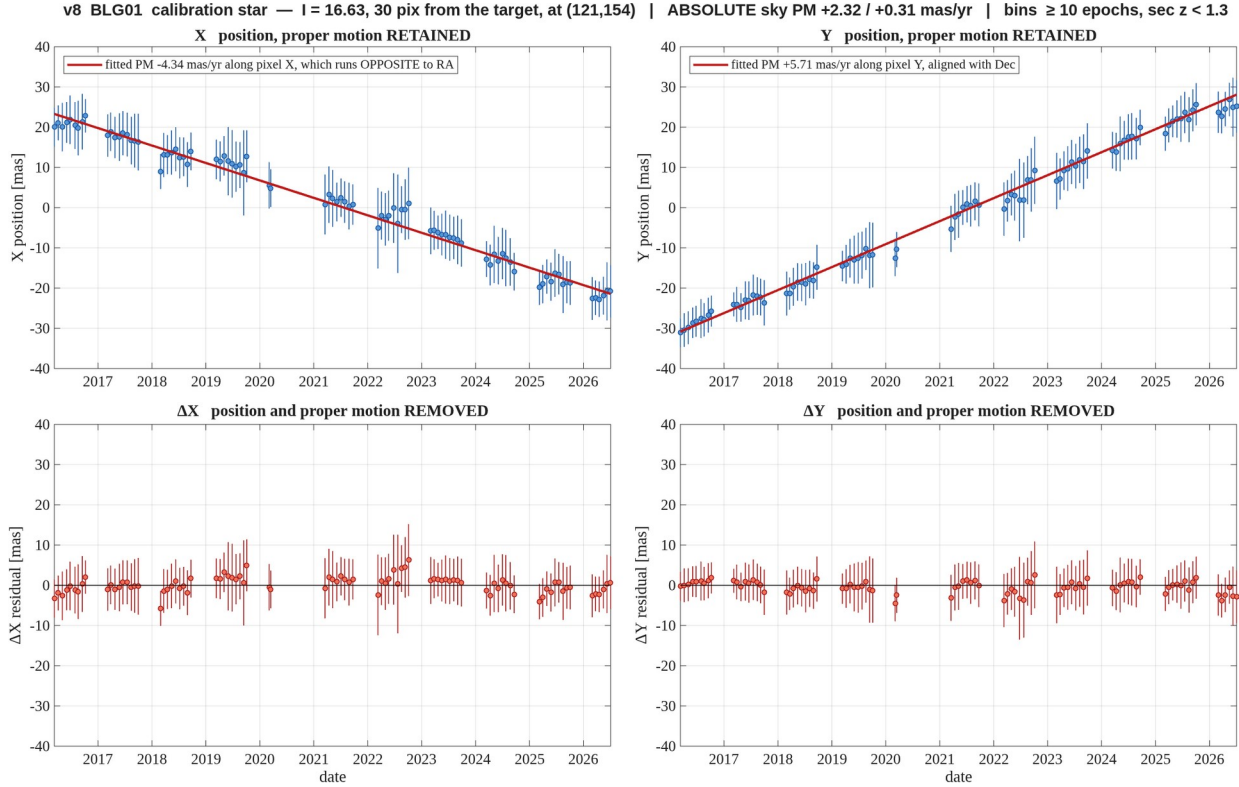
Figure 21. BLG01 — l = 16.63 , 30 pix away. Binned in one sidereal month, error bars are the RMS within the bin; bins with fewer than 10 epochs and epochs at sec z > 1.3 are dropped. Columns are the two axes, X left and Y right ; the top row keeps the proper motion, the bottom row removes it. The heading gives the absolute sky motion with the full gauge removed; the legend gives it along the pixel axis, and pixel X runs opposite to RA , so the two carry opposite signs in X.
