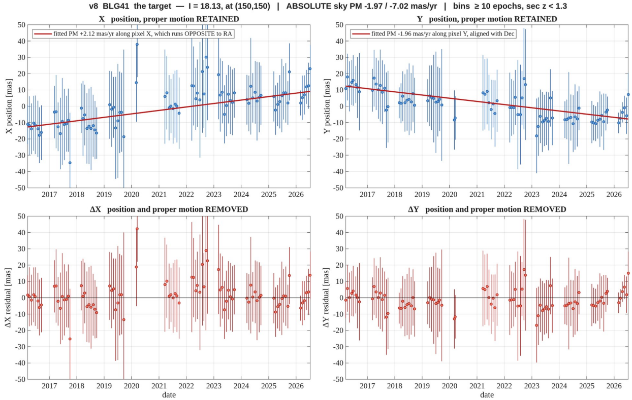
Figure 9. BLG41 — the target, l = 18.13 . Binned in one sidereal month, error bars are the RMS within the bin; bins with fewer than 10 epochs and epochs at \sec z > 1.3 are dropped. Columns are the two axes, X left and Y right ; the top row keeps the proper motion, the bottom row removes it. The heading gives the absolute sky motion with the full gauge removed; the legend gives it along the pixel axis, and pixel X runs opposite to RA , so the two carry opposite signs in X. report_v8_motion_BLG41_target.png
