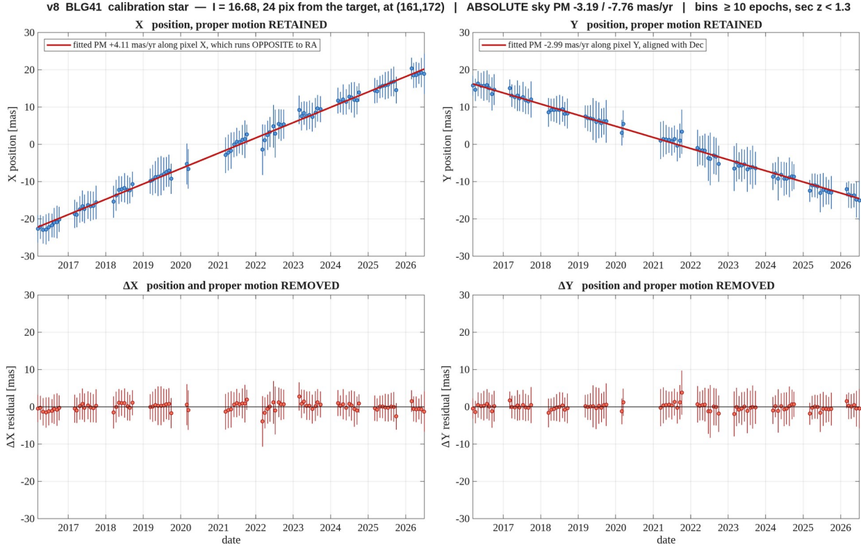
Figure 13. BLG41 — l = 16.68 , 24 pix away. Binned in one sidereal month, error bars are the RMS within the bin; bins with fewer than 10 epochs and epochs at sec z > 1.3 are dropped. Columns are the two axes, X left and Y right ; the top row keeps the proper motion, the bottom row removes it. The heading gives the absolute sky motion with the full gauge removed; the legend gives it along the pixel axis, and pixel X runs opposite to RA , so the two carry opposite signs in X.
