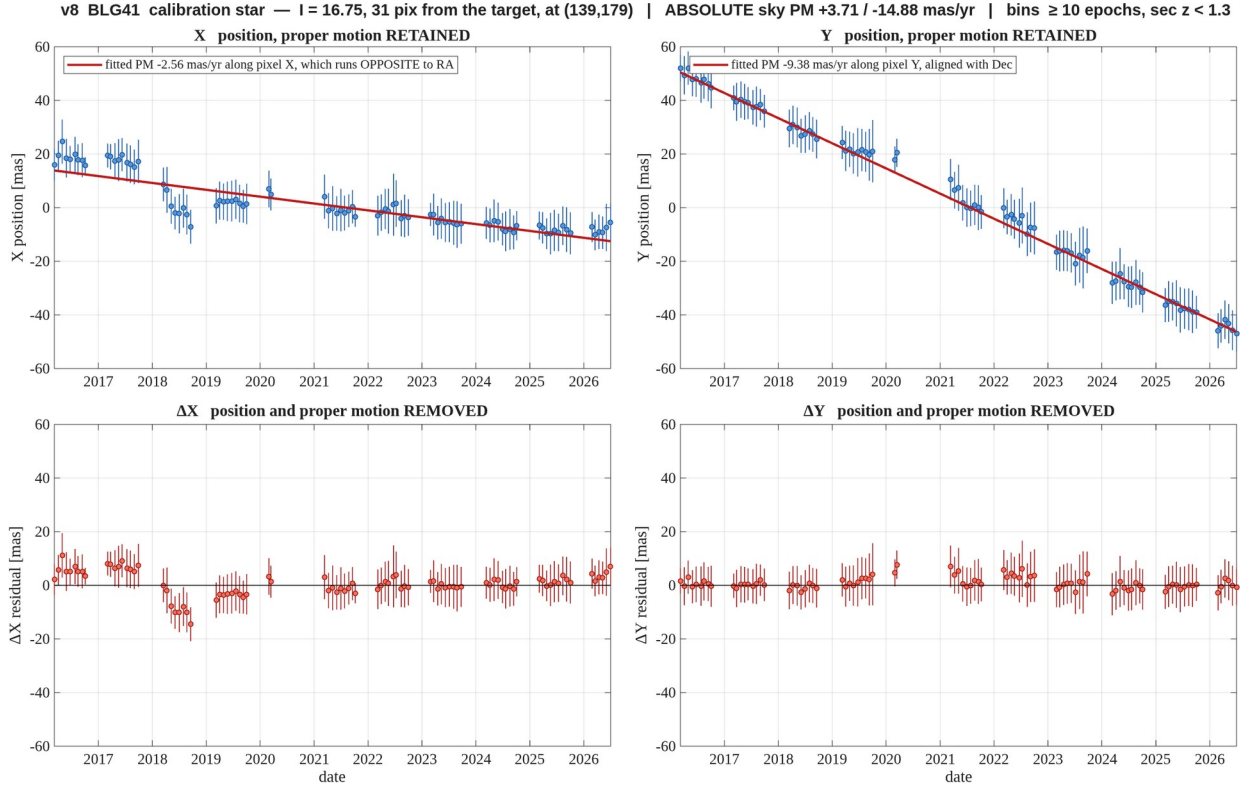
Figure 15. BLG41 — l = 16.75 , 31 pix away. Binned in one sidereal month, error bars are the RMS within the bin; bins with fewer than 10 epochs and epochs at sec z > 1.3 are dropped. Columns are the two axes, X left and Y right ; the top row keeps the proper motion, the bottom row removes it. The heading gives the absolute sky motion with the full gauge removed; the legend gives it along the pixel axis, and pixel X runs opposite to RA , so the two carry opposite signs in X.
