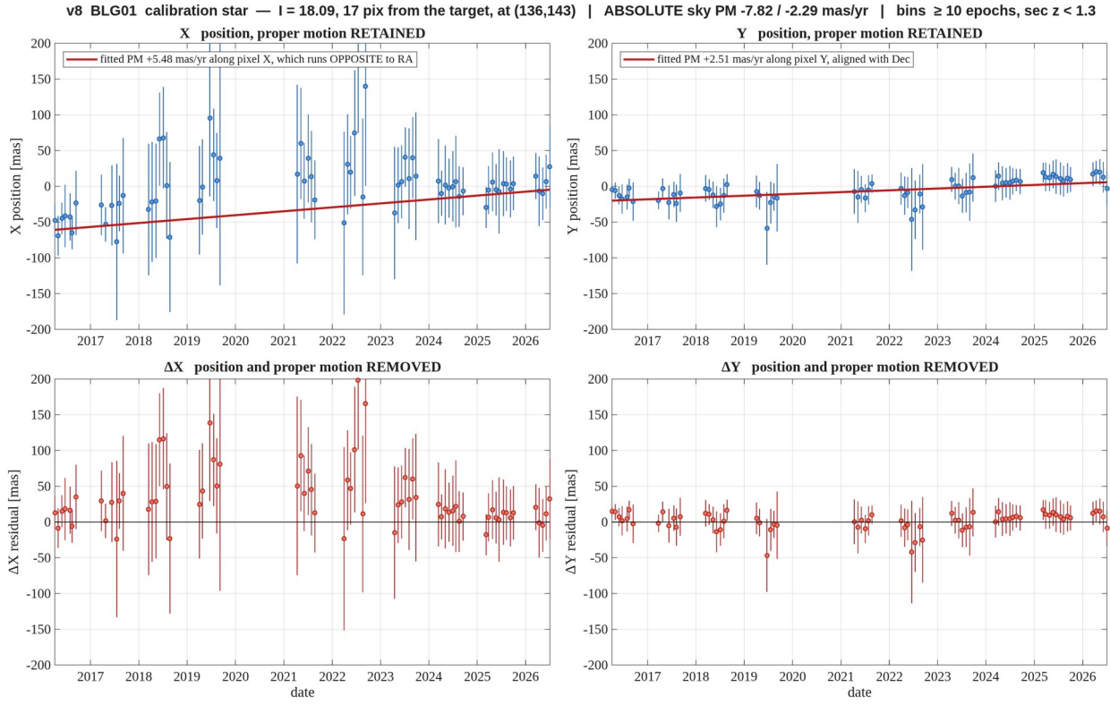
Figure 18. BLG01 — l = 18.09 , 17 pix away — poorly measured, see section 7. Binned in one sidereal month, error bars are the RMS within the bin; bins with fewer than 10 epochs and epochs at sec z > 1.3 are dropped. Columns are the two axes, X left and Y right ; the top row keeps the proper motion, the bottom row removes it. The heading gives the absolute sky motion with the full gauge removed; the legend gives it along the pixel axis, and pixel X runs opposite to RA , so the two carry opposite signs in X. report_v8_motion_BLG01_m18_d17.png
