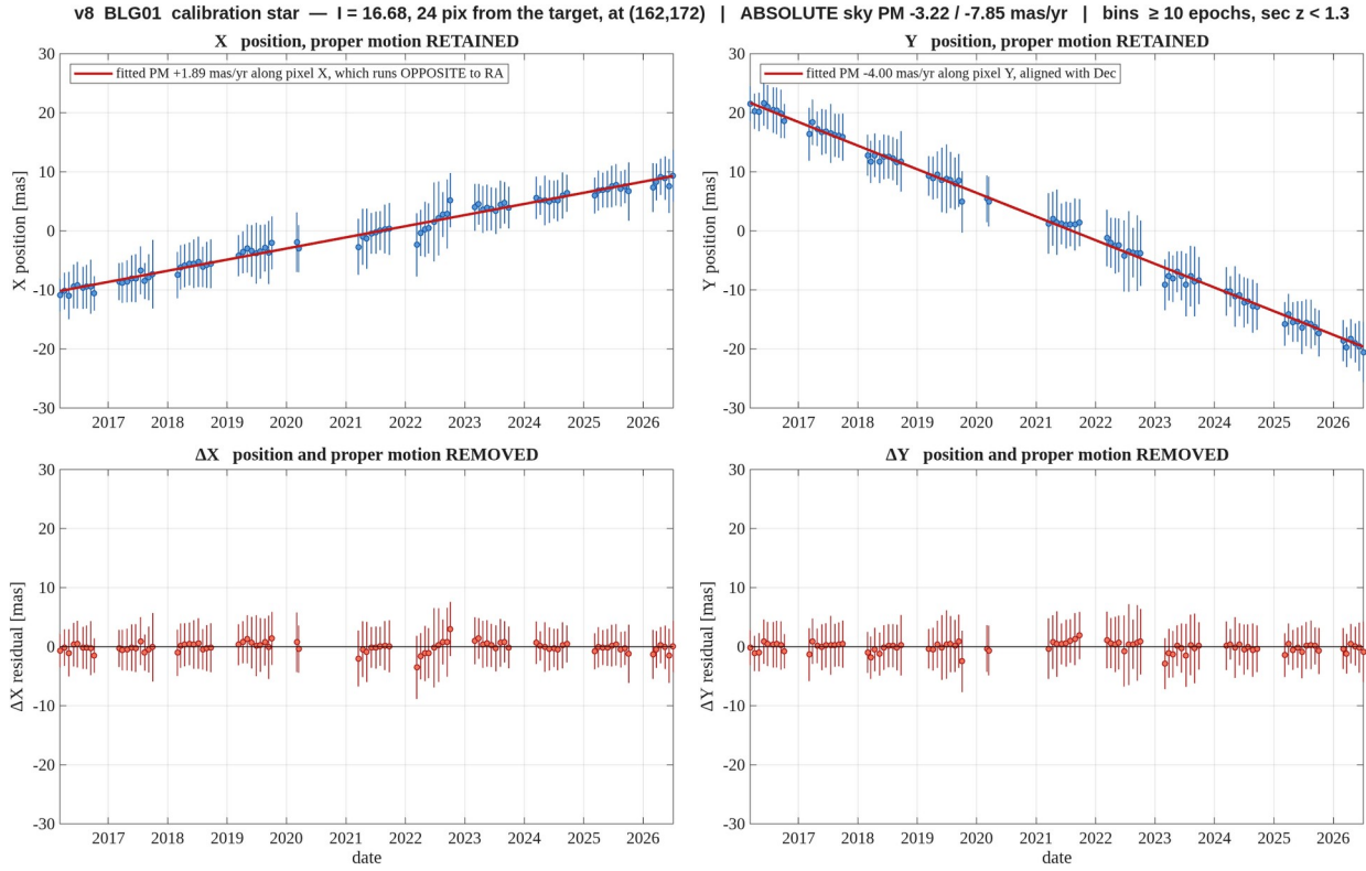
Figure 20. BLG01 — l = 16.68 , 24 pix away. Binned in one sidereal month, error bars are the RMS within the bin; bins with fewer than 10 epochs and epochs at sec z > 1.3 are dropped. Columns are the two axes, X left and Y right ; the top row keeps the proper motion, the bottom row removes it. The heading gives the absolute sky motion with the full gauge removed; the legend gives it along the pixel axis, and pixel X runs opposite to RA , so the two carry opposite signs in X.
