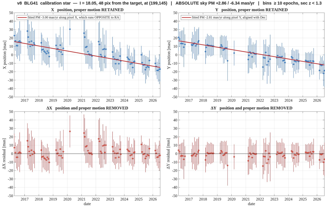
Figure 12. BLG41 — l = 18.05 , 48 pix away. Binned in one sidereal month, error bars are the RMS within the bin; bins with fewer than 10 epochs and epochs at sec z > 1.3 are dropped. Columns are the two axes, X left and Y right ; the top row keeps the proper motion, the bottom row removes it. The heading gives the absolute sky motion with the full gauge removed; the legend gives it along the pixel axis, and pixel X runs opposite to RA , so the two carry opposite signs in X.
