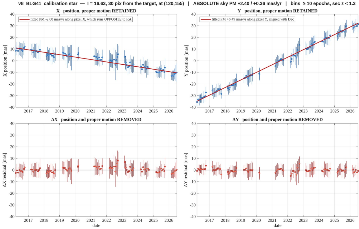
Figure 14. BLG41 — l = 16.63 , 30 pix away. Binned in one sidereal month, error bars are the RMS within the bin; bins with fewer than 10 epochs and epochs at sec z > 1.3 are dropped. Columns are the two axes, X left and Y right ; the top row keeps the proper motion, the bottom row removes it. The heading gives the absolute sky motion with the full gauge removed; the legend gives it along the pixel axis, and pixel X runs opposite to RA , so the two carry opposite signs in X.
