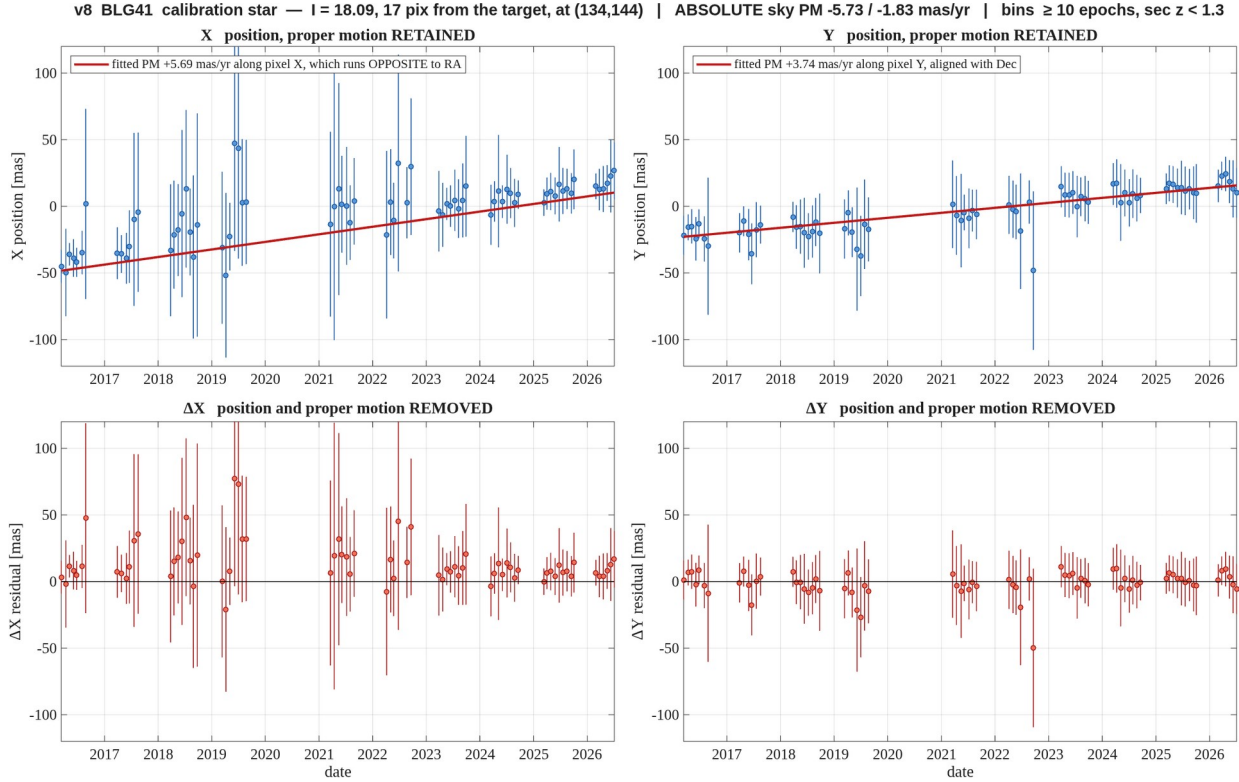
Figure 11. BLG41 — l = 18.09 , 17 pix away — poorly measured , see section 7. Binned in one sidereal month, error bars are the RMS within the bin; bins with fewer than 10 epochs and epochs at sec z > 1.3 are dropped. Columns are the two axes, X left and Y right ; the top row keeps the proper motion, the bottom row removes it. The heading gives the absolute sky motion with the full gauge removed; the legend gives it along the pixel axis, and pixel X runs opposite to RA , so the two carry opposite signs in X. report_v8_motion_BLG41_m18_d17.png
