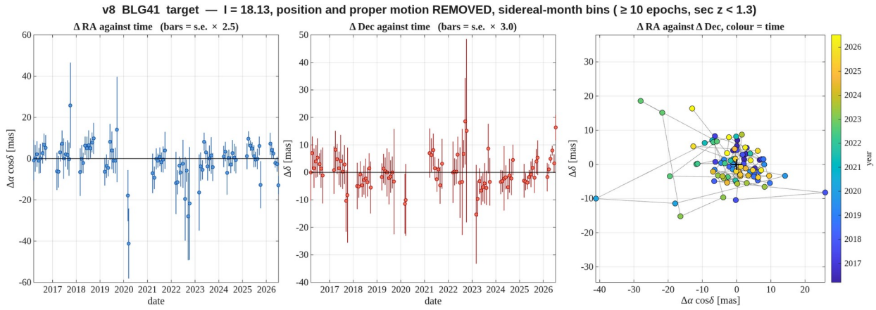
Figure 3. BLG41 — the target, l = 18.13 . Position and proper motion removed: these are the residuals. Left: RA residual against time. Middle: Dec residual against time. Right: the two against each other with time colour-coded, where a well-behaved star shows an unordered cloud about the origin and any systematic drift would appear as an ordered progression of colour; consecutive months are joined by a thin grey line. Sidereal-month bins; error bars are the standard error within the bin scaled by the empirical factor \sqrt{(\chi^2/\text{DoF})} of the bin means, quoted in each panel title, so that they carry the real bin-to-bin scatter (section 7). Bins with fewer than 10 epochs and epochs at \sec z > 1.3 are dropped: the season-edge months, with a handful of high-airmass frames, otherwise dominate the plot.
