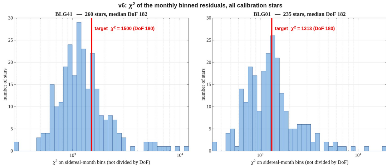
Figure 2. \chi^2 of the sidereal-month binned residuals for every calibration star, both axes combined, not divided by DoF . Each bin contributes (mean / standard error) 2 per axis and DoF = 2N bins – 4. The red line marks the target, which sits in the body of the distribution rather than the tail.
