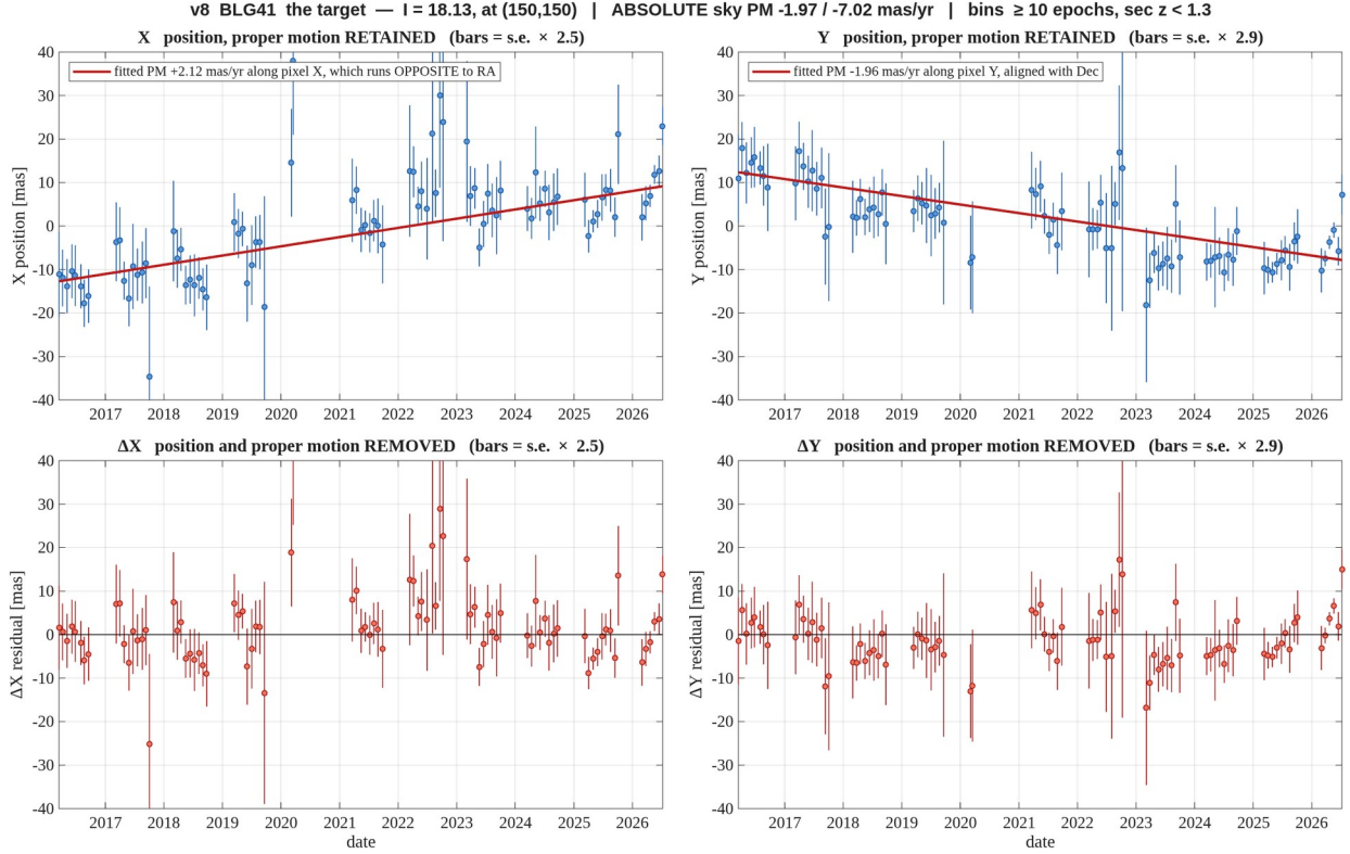
Figure 9. BLG41 — the target, I = 18.13. Binned in one sidereal month, error bars are the standard error within the bin scaled by the empirical factor \sqrt{\chi^2/\text{DoF}} of the bin means (quoted in the panel titles, computed on the proper-motion-removed residuals and applied to both rows); bins with fewer than 10 epochs and epochs at \sec z > 1.3 are dropped. Columns are the two axes, X left and Y right ; the top row keeps the proper motion, the bottom row removes it. The heading gives the absolute sky motion with the full gauge removed; the legend gives it along the pixel axis, and pixel X runs opposite to RA , so the two carry opposite signs in X.
