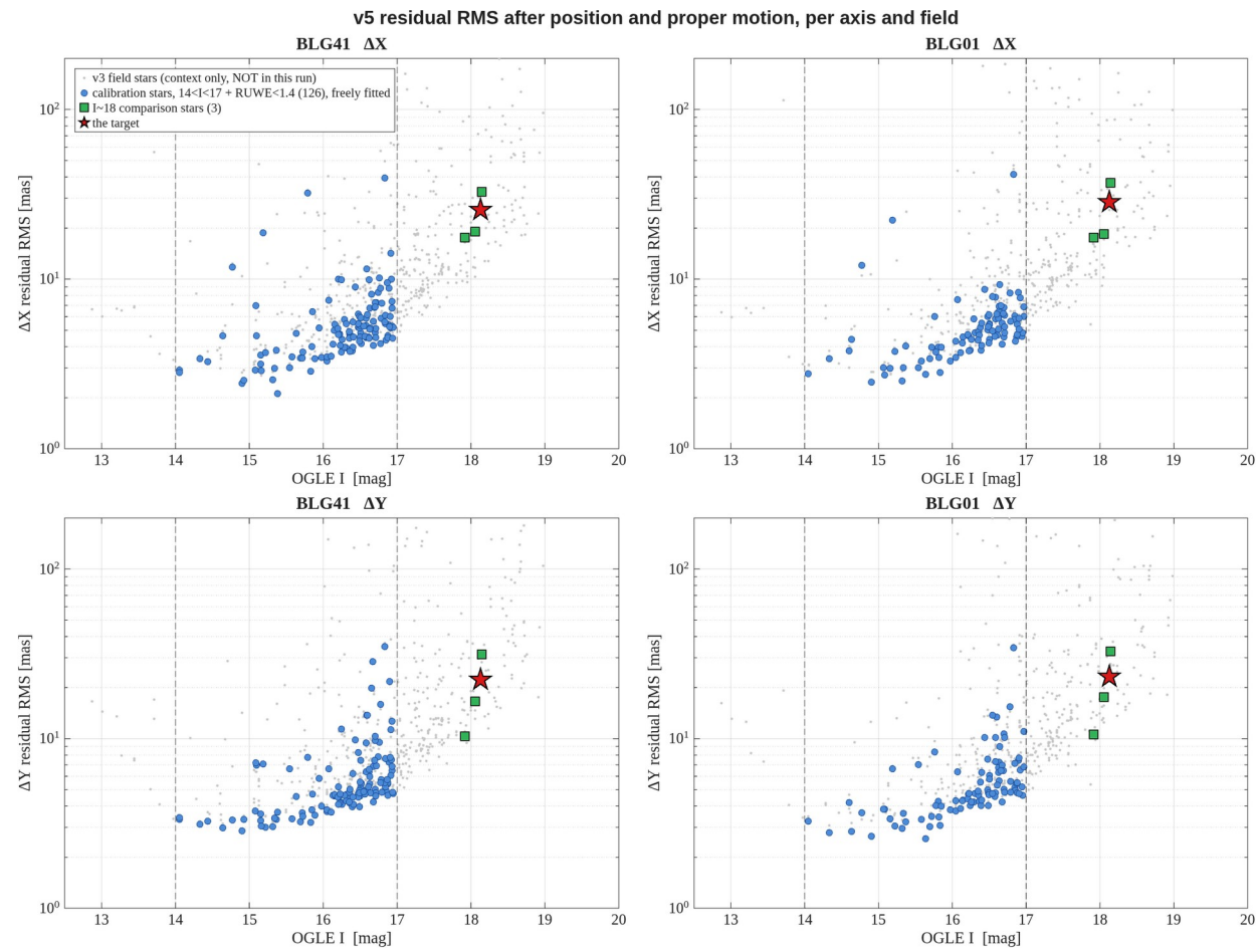
Figure 1. Residual RMS against the OGLE catalogue magnitude, per axis and per field, for the v5 run, after position and proper motion have been removed. Blue: the 126 / 96 calibration stars, 14<I<17 with RUWE<1.4, freely fitted . Green: the three 1~18 comparison stars. Red: the target. Grey: field stars from the reference reduction, shown for context only — they are not part of this run . Dashed lines mark the 14 and 17 mag limits.
