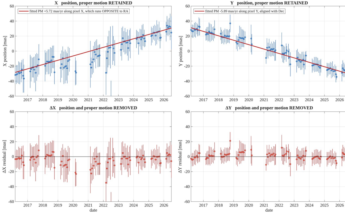
Figure 28. v5, BLG01 — passenger at the target magnitude, 21 pix away, freely fitted. The same star as the corresponding v4 figure, but from the run in which nothing is pinned and Gaia enters only as a post-hoc tie. Sky motions quoted in the heading have the gauge removed and are absolute. Binned in one sidereal month; columns are the two axes, X left and Y right; top row keeps the proper motion, bottom row removes it. Pixel X runs opposite to RA , so the legend and the heading carry opposite signs in X. report_v5_motion_BLG01_out_d21.png
