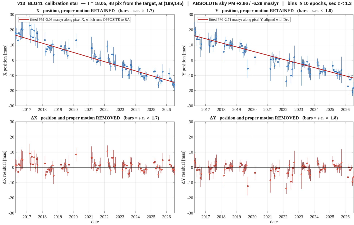
Figure 12. BLG41 — I = 18.05 , 48 pix away. Binned in one sidereal month, error bars are the standard error within the bin scaled by the empirical factor \sqrt{(\chi^2/\text{DoF})} of the bin means (quoted in the panel titles, computed on the proper-motion-removed residuals and applied to both rows); bins with fewer than 10 epochs and epochs at \text{sec } z > 1.3 are dropped. Columns are the two axes, X left and Y right ; the top row keeps the proper motion, the bottom row removes it. The heading gives the absolute sky motion with the full gauge removed; the legend gives it along the pixel axis, and pixel X runs opposite to RA , so the two carry opposite signs in X.
