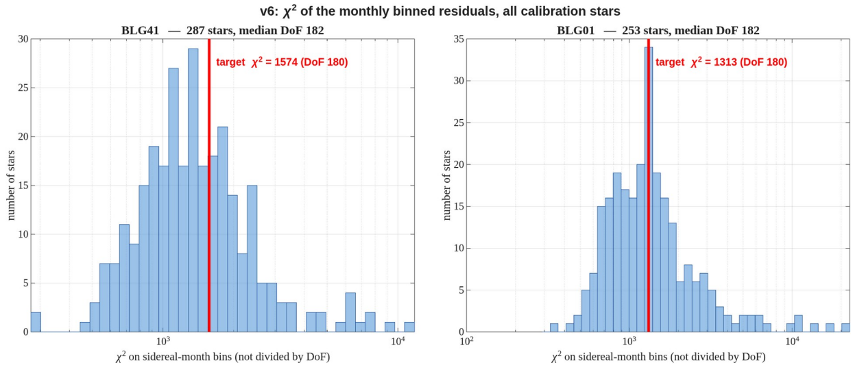
Figure 3. \chi^2 of the sidereal-month binned residuals for every calibration star, both axes combined, not divided by DoF . Each bin contributes (mean / standard error) 2 per axis and \text{DoF} = 2N_{\text{bins}} - 4 . The red line marks the target, which sits in the body of the distribution rather than the tail. report_v6_chi2.png
