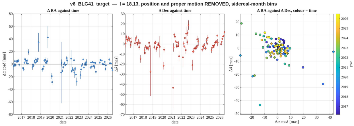
Figure 4. BLG41 — the target, l = 18.13 . Position and proper motion removed : these are the residuals. Left: RA residual against time. Middle: Dec residual against time. Right: the two against each other with time colour-coded, where a well-behaved star shows an unordered cloud about the origin and any systematic drift would appear as an ordered progression of colour. Sidereal-month bins; error bars are the standard error within the bin, which section 8 shows understates the true scatter by about 2.6. report_v6_radec_BLG41_target.png
