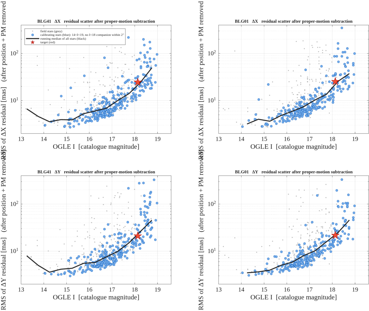
Figure 1. Residual RMS against the OGLE catalogue magnitude, per axis and per field, after position and proper motion have been removed . Grey: all field stars. Blue: calibrating stars (14<l<19, no l<18 companion within 2 arcsec). Black: running median of all stars, the curve the CSV decade errors are read from. Red: the target. report_RMS_afterPM.png
