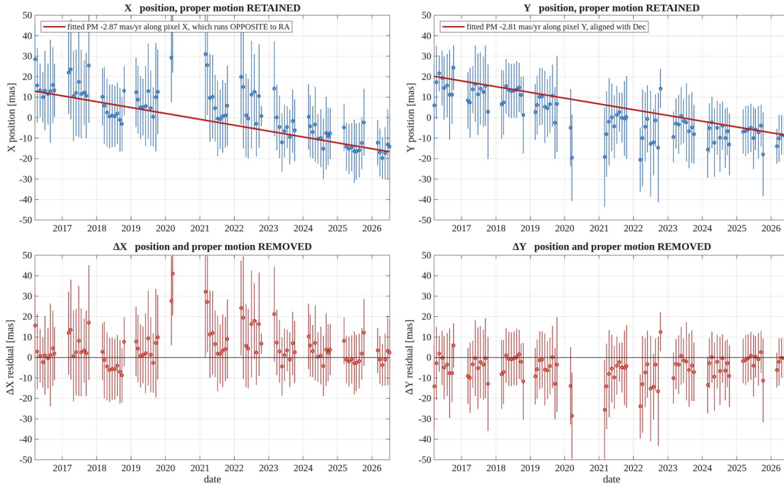
Figure 8. BLG41 — comparison star l = 18.05 , 48 pix away. Every star here is freely fitted; nothing is pinned. Binned in one sidereal month, error bars are the RMS within the bin. Columns are the two axes, X left and Y right ; the top row keeps the proper motion, the bottom row removes it. The heading gives the absolute sky motion with the gauge removed; the legend gives it along the pixel axis, and pixel X runs opposite to RA , so the two carry opposite signs in X.
