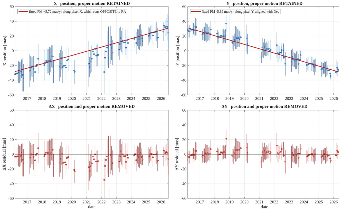
Figure 14. BLG01 — comparison star l = 17.91, 21 pix away. Every star here is freely fitted; nothing is pinned. Binned in one sidereal month, error bars are the RMS within the bin. Columns are the two axes, X left and Y right ; the top row keeps the proper motion, the bottom row removes it. The heading gives the absolute sky motion with the gauge removed; the legend gives it along the pixel axis, and pixel X runs opposite to RA , so the two carry opposite signs in X.
