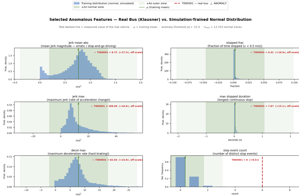
Figure 13: Six selected features of the real Klausner bus (T000001, red dashed line) against the distribution of the same features over 13,333 simulated normal tracks. Shaded bands mark the \pm 2\sigma and \pm 4\sigma zones about the training mean \mu ; values beyond the plotted window are annotated with their Z-score. The anomaly threshold is |z| > 15.4 .
