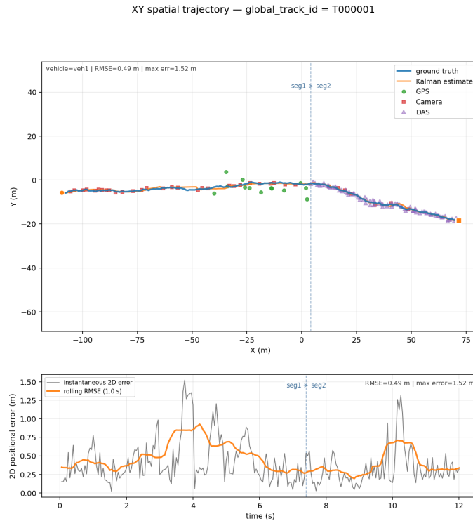
Figure 7: Fused multi-sensor track versus ground truth for a cross-segment vehicle. Top: spatial trajectory with DAS, camera, and GPS measurements, and the dashed line marks the segment boundary. Bottom: instantaneous and rolling 2-D error (RMSE = 0.49 m, max 1.52 m).
