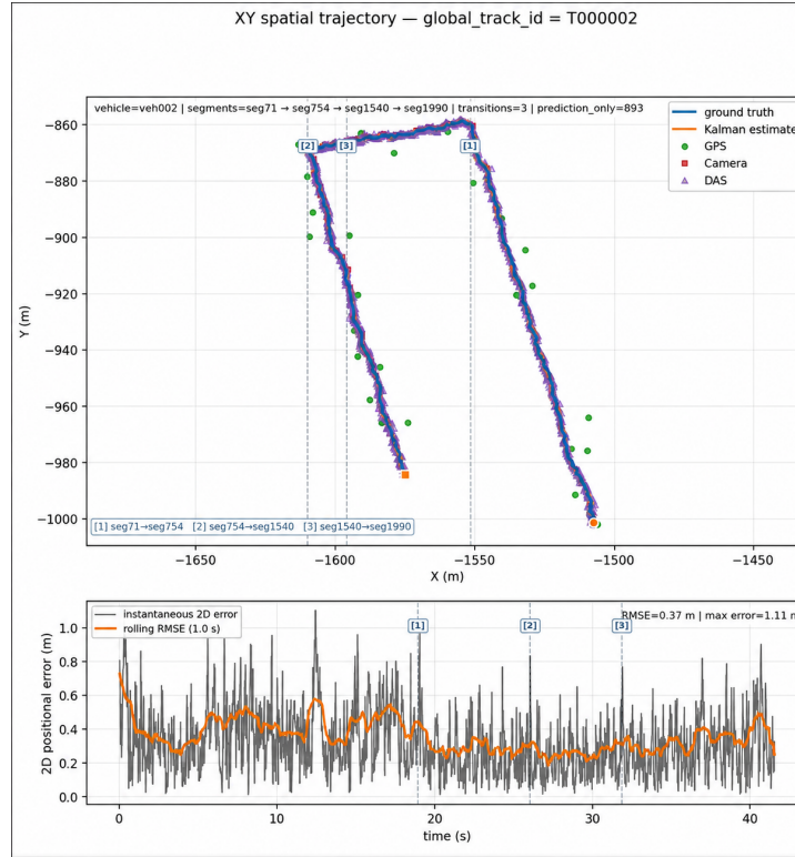
Figure 8: Continuous tracking across four connected segments (over-speeding scenario). Top: spatial trajectory with DAS, camera, and GPS measurements and three segment transitions. Bottom: 2-D error over time (RMSE = 0.37 m, max error = 1.11 m).
