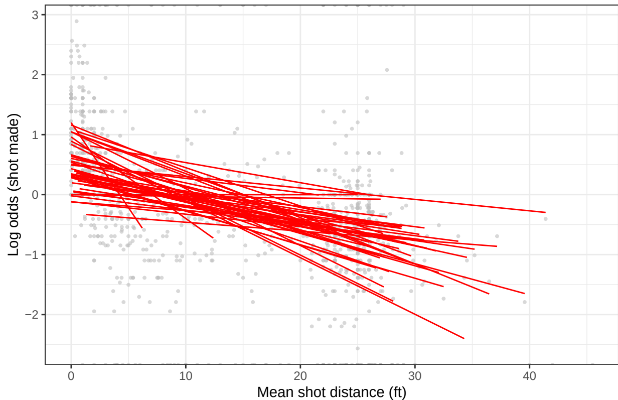
Spaghetti Plot of 50 Random NBA players logodds against binned shot distance
