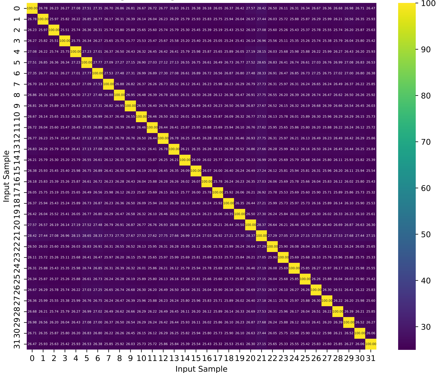
Matching Percentages of Activation Patterns (GPU)
