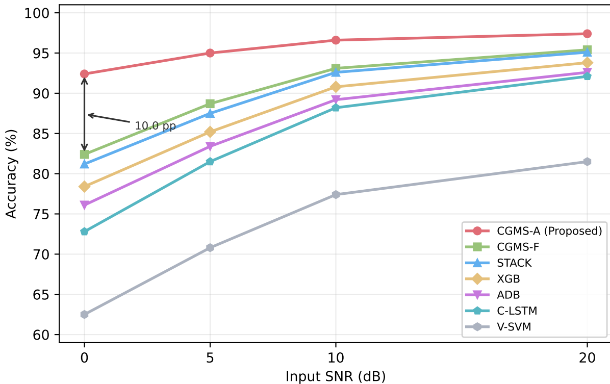
Accuracy vs Input SNR — ICMPRS Synthetic Benchmark (All curves from synthetic data; real-cohort performance will differ)
