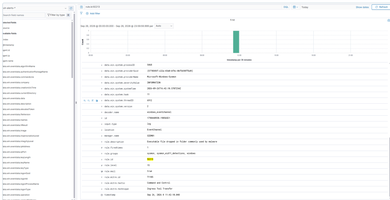
Figure 20.2: Rule 92213, "Executable file dropped in folder commonly used by malware", firing at
