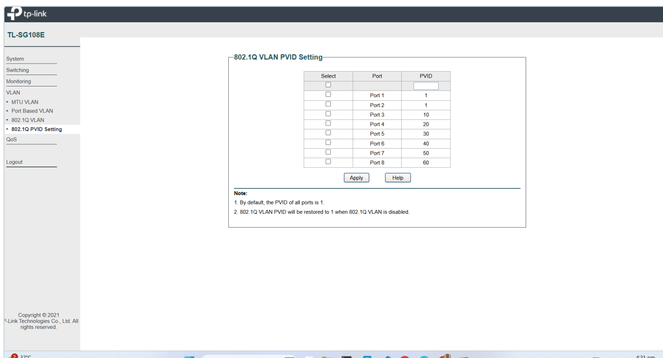
Figure 1.5 — 802.1Q PVID settings. Each access port 3–8 carries the PVID of its VLAN (10, 20, 30, 40, 50, 60), so any untagged device plugged in lands in the correct segment automatically. Trunk ports 1–2 keep PVID 1 because they only ever carry tagged traffic. Figures 1.4 and 1.5 together are the switch-side proof of the port map in the table above, and they mirror the pfSense sub-interfaces in Figure 1.1.
